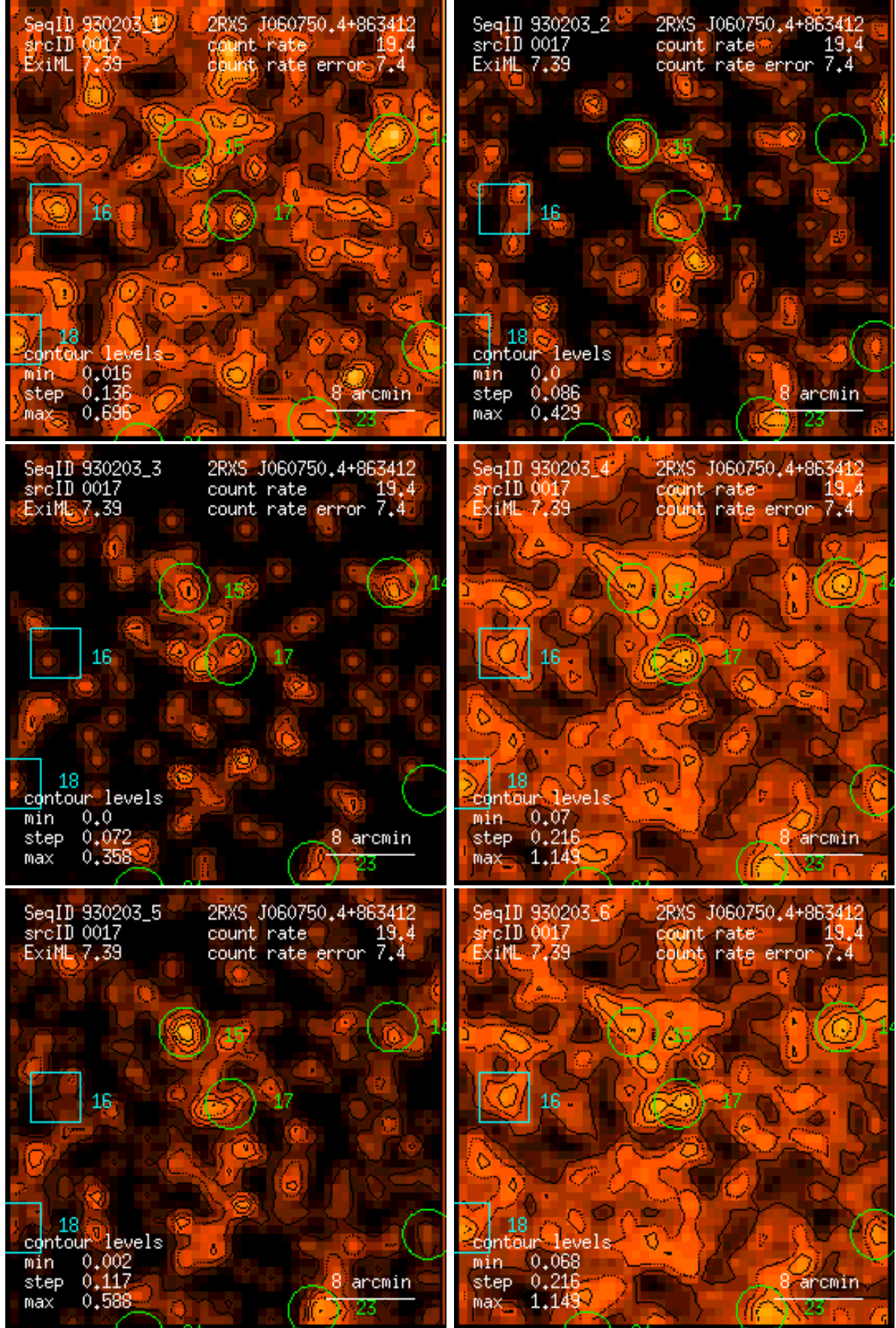
Figure 17: RASS 930203: detection 0017: band rate images, Gaussian filter: (1) PSPC channels 11 – 41, (2) 52 – 90, (3) 91 – 201, (4) 11 – 235, (5) 52 – 201, (6) 11 – 201. Broad band rates in counts/ks. Band rate contour levels in counts/ks/arcmin 2 .
