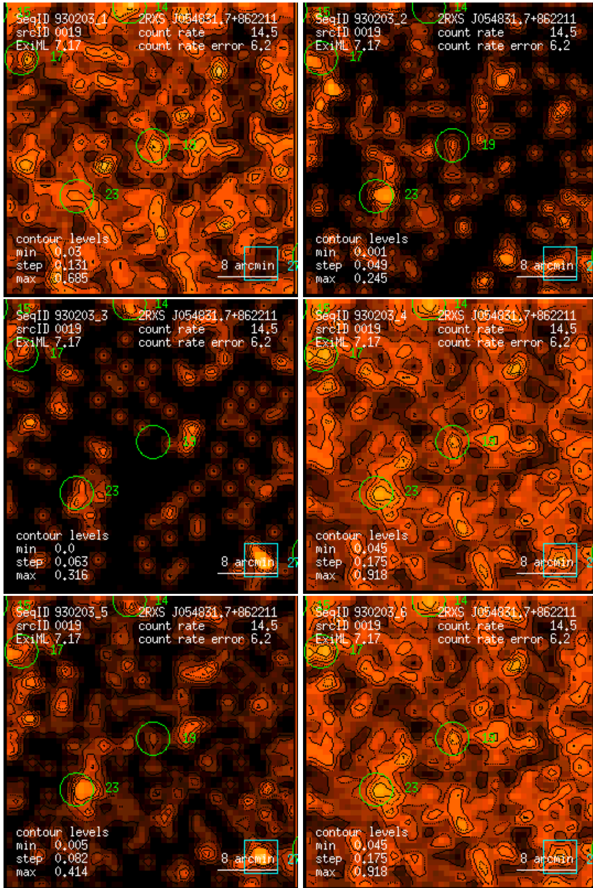
Figure 19: RASS 930203: detection 0019: band rate images, Gaussian filter: (1) PSPC channels 11 – 41, (2) 52 – 90, (3) 91 – 201, (4) 11 – 235, (5) 52 – 201, (6) 11 – 201. Broad band rates in counts/ks. Band rate contour levels in counts/ks/arcmin 2 .
