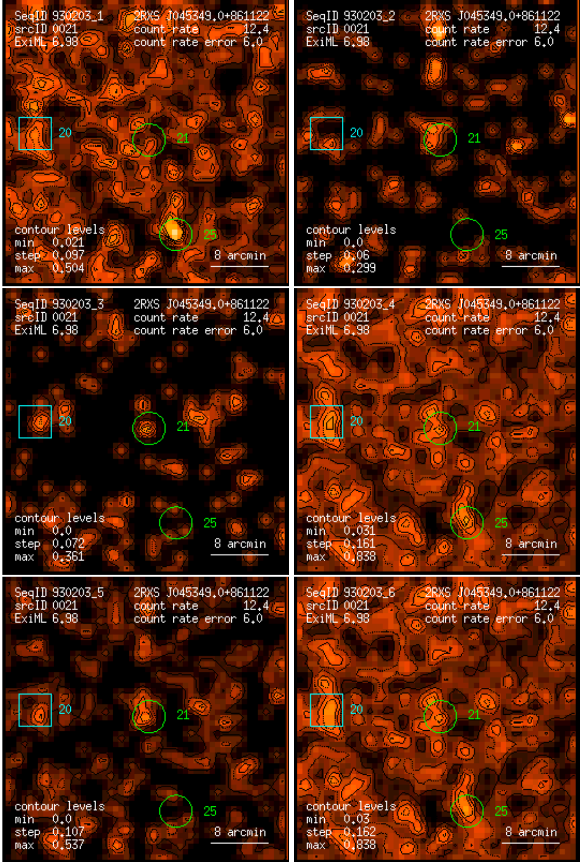
Figure 21: RASS 930203: detection 0021: band rate images, Gaussian filter: (1) PSPC channels 11 – 41, (2) 52 – 90, (3) 91 – 201, (4) 11 – 235, (5) 52 – 201, (6) 11 – 201. Broad band rates in counts/ks. Band rate contour levels in counts/ks/arcmin 2 .
