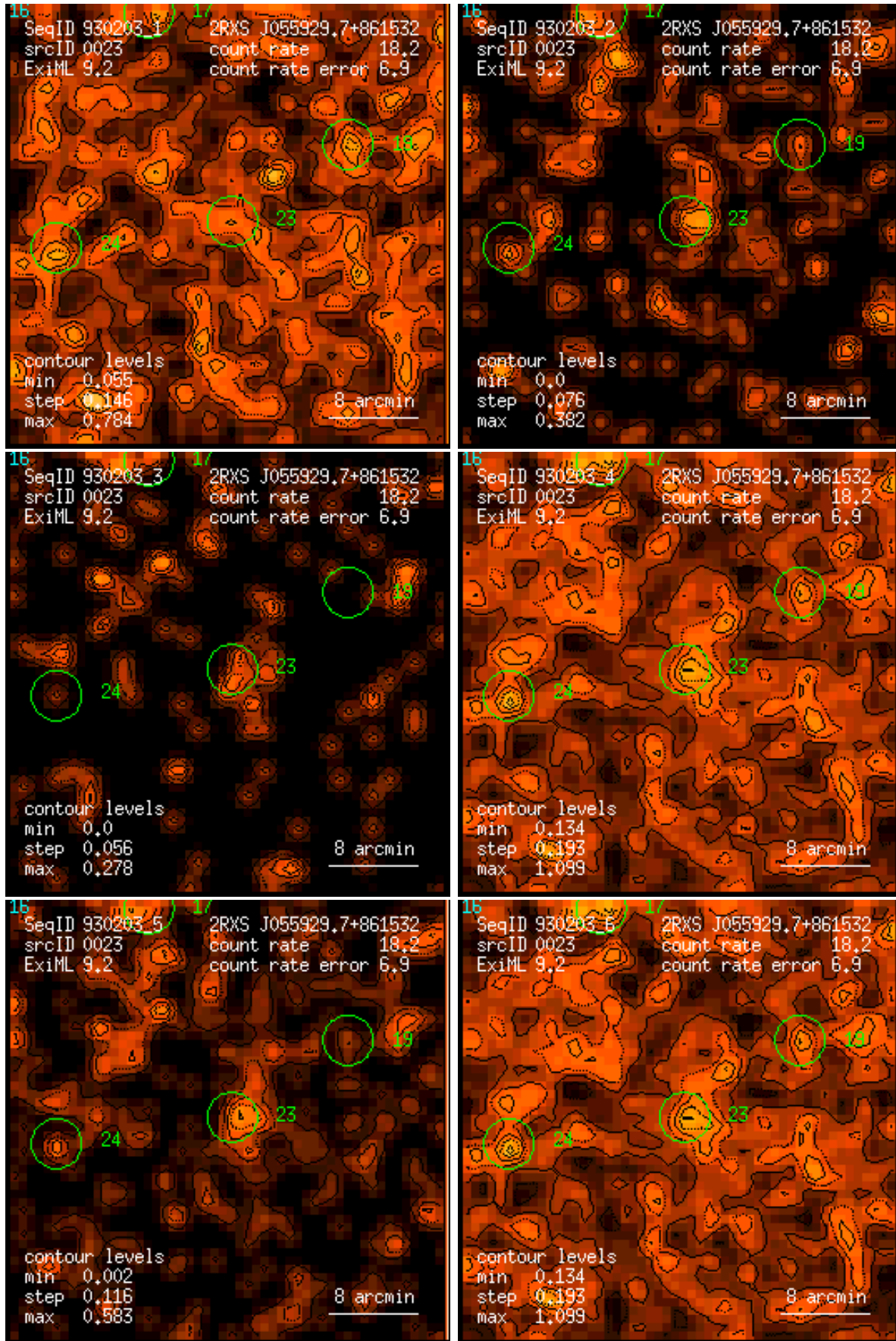
Figure 23: RASS 930203: detection 0023: band rate images, Gaussian filter: (1) PSPC channels 11 – 41, (2) 52 – 90, (3) 91 – 201, (4) 11 – 235, (5) 52 – 201, (6) 11 – 201. Broad band rates in counts/ks. Band rate contour levels in counts/ks/arcmin 2 .
