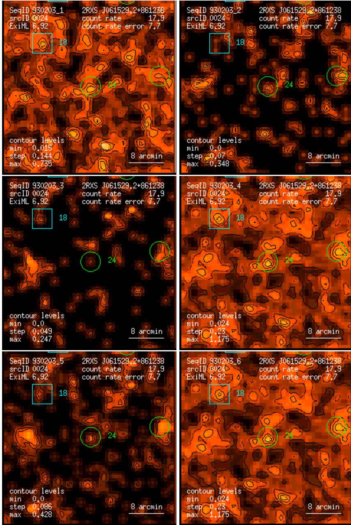
Figure 24: RASS 930203: detection 0024: band rate images, Gaussian filter: (1) PSPC channels 11 – 41, (2) 52 – 90, (3) 91 – 201, (4) 11 – 235, (5) 52 – 201, (6) 11 – 201. Broad band rates in counts/ks. Band rate contour levels in counts/ks/arcmin 2 .
