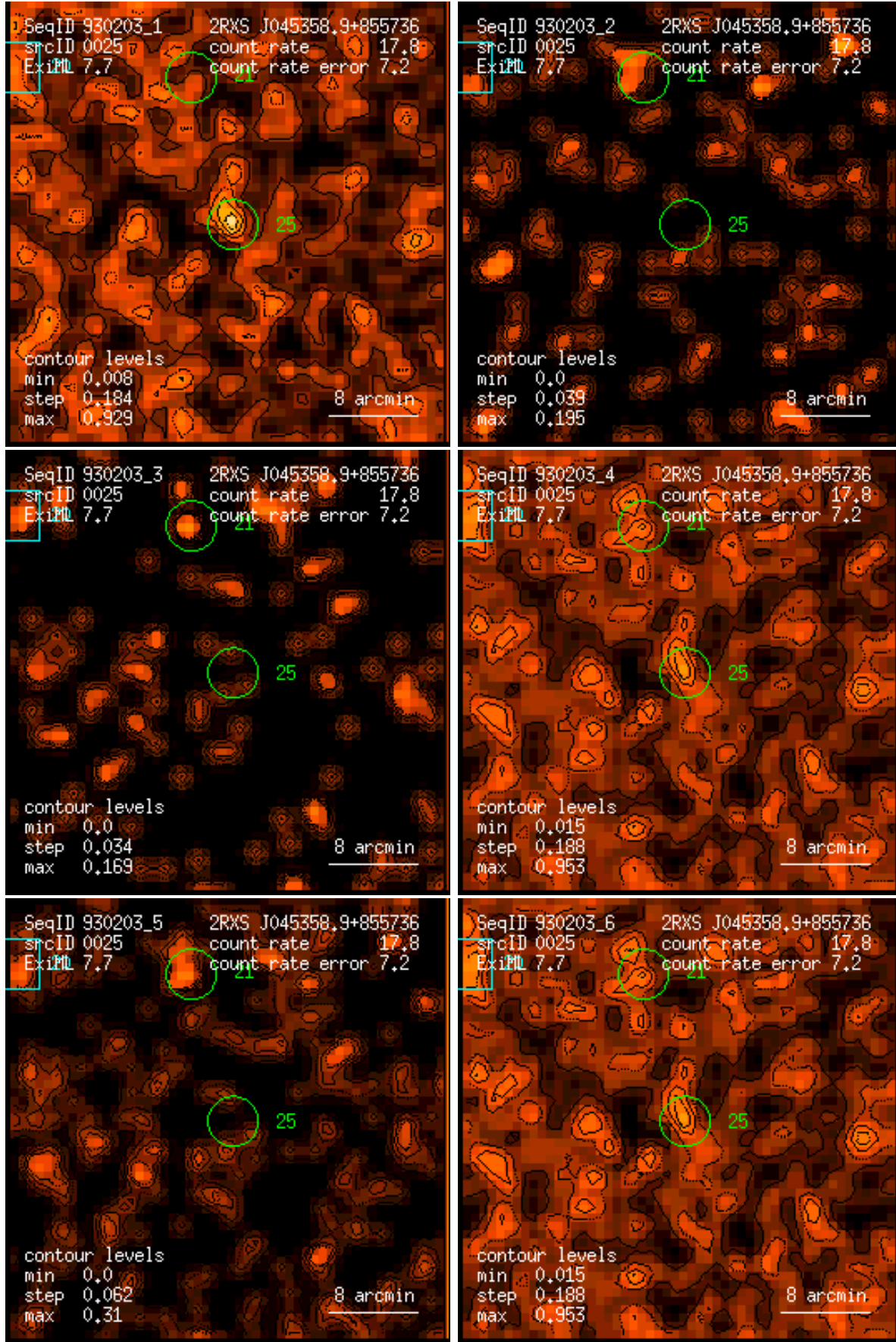
Figure 25: RASS 930203: detection 0025: band rate images, Gaussian filter: (1) PSPC channels 11 – 41, (2) 52 – 90, (3) 91 – 201, (4) 11 – 235, (5) 52 – 201, (6) 11 – 201. Broad band rates in counts/ks. Band rate contour levels in counts/ks/arcmin 2 .
