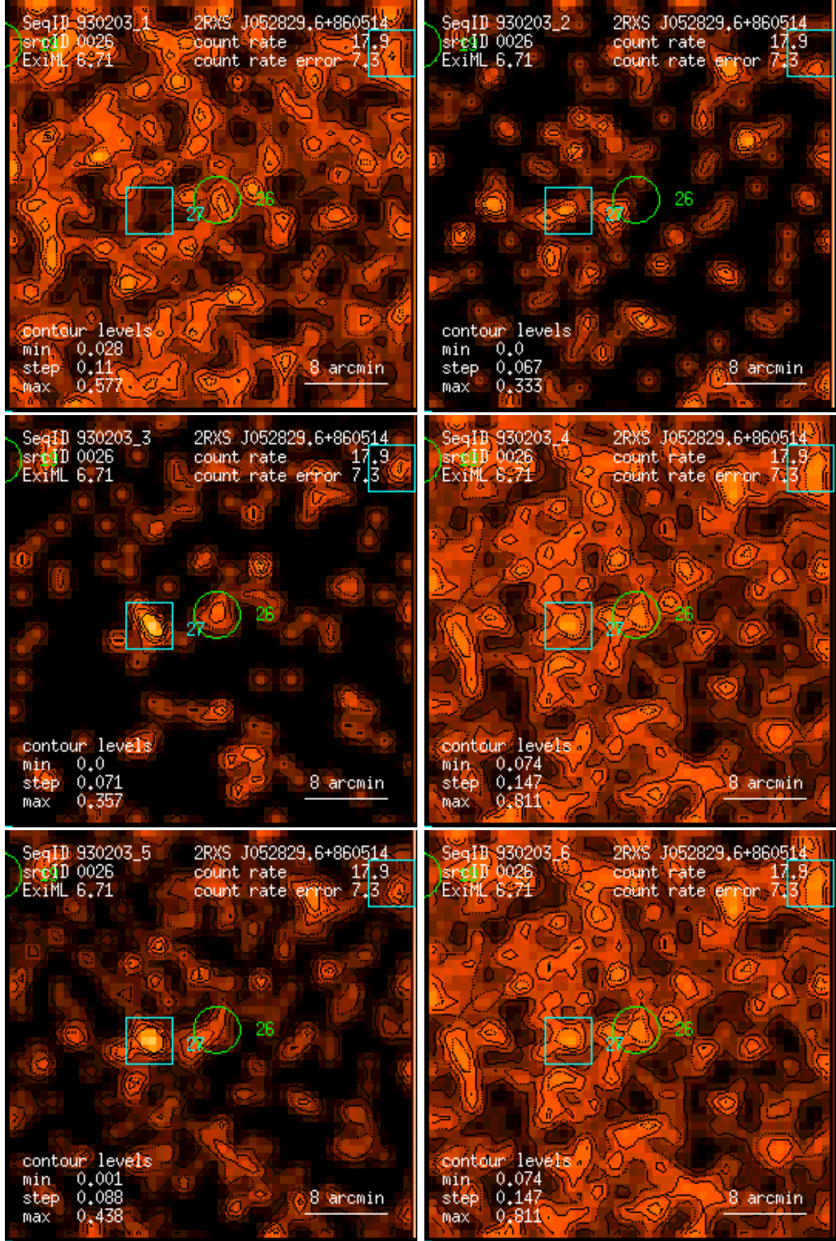
Figure 26: RASS 930203: detection 0026: band rate images, Gaussian filter: (1) PSPC channels 11 – 41, (2) 52 – 90, (3) 91 – 201, (4) 11 – 235, (5) 52 – 201, (6) 11 – 201. Broad band rates in counts/ks. Band rate contour levels in counts/ks/arcmin 2 .
