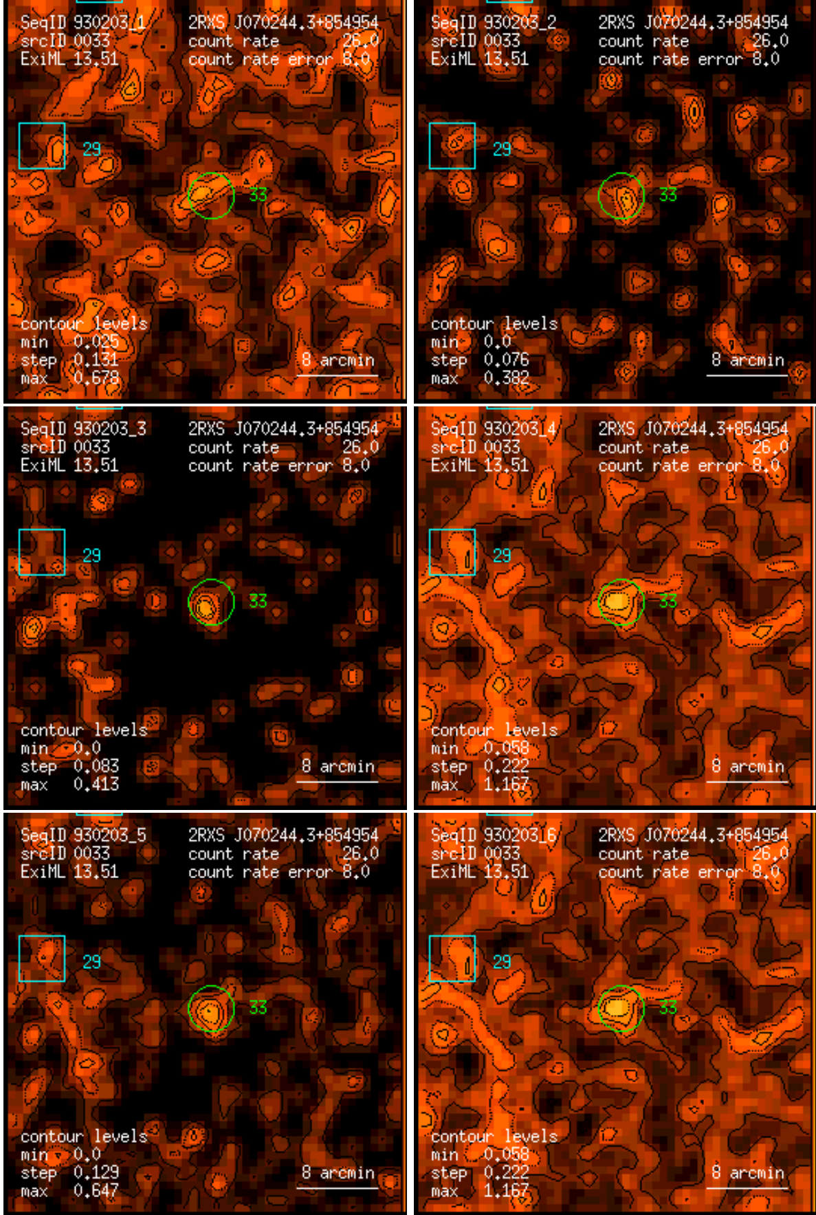
Figure 33: RASS 930203: detection 0033: band rate images, Gaussian filter: (1) PSPC channels 11 – 41, (2) 52 – 90, (3) 91 – 201, (4) 11 – 235, (5) 52 – 201, (6) 11 – 201. Broad band rates in counts/ks. Band rate contour levels in counts/ks/arcmin 2 .
