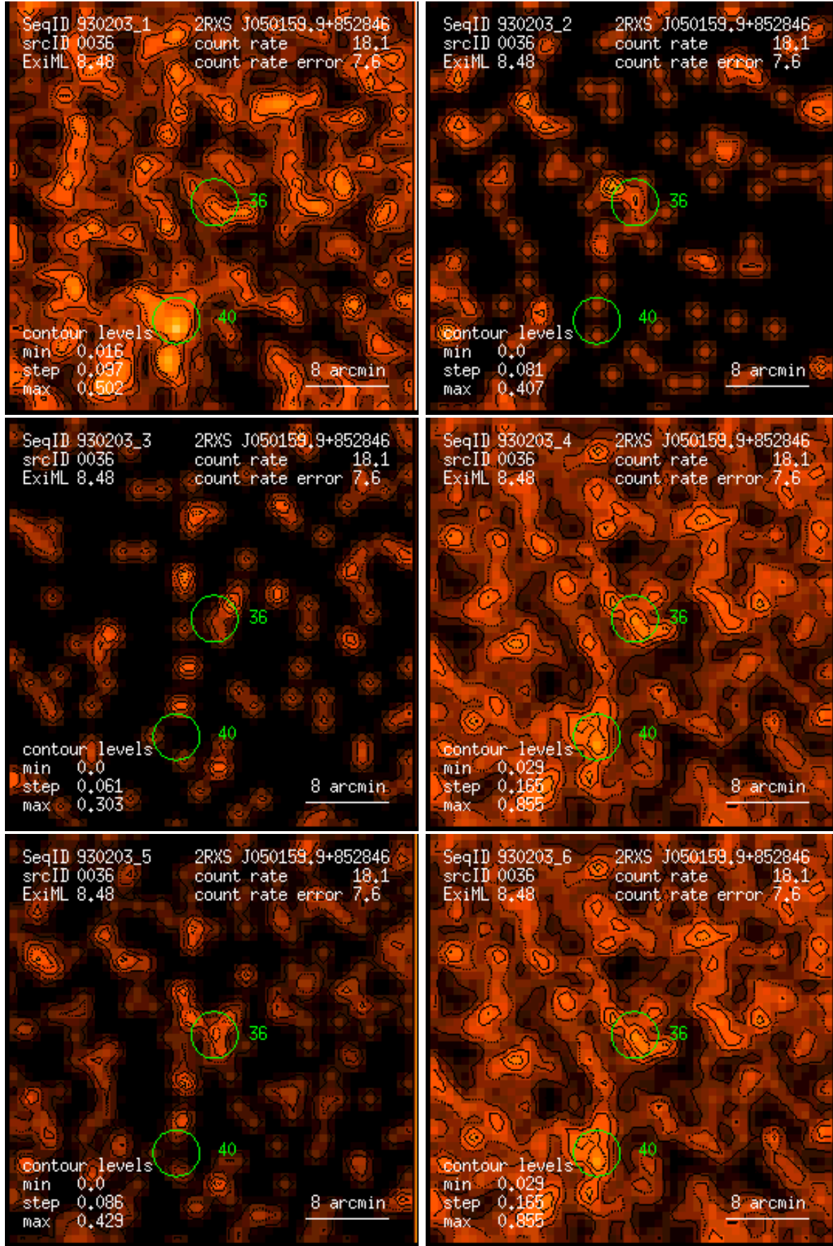
Figure 36: RASS 930203: detection 0036: band rate images, Gaussian filter: (1) PSPC channels 11 – 41, (2) 52 – 90, (3) 91 – 201, (4) 11 – 235, (5) 52 – 201, (6) 11 – 201. Broad band rates in counts/ks. Band rate contour levels in counts/ks/arcmin 2 .
