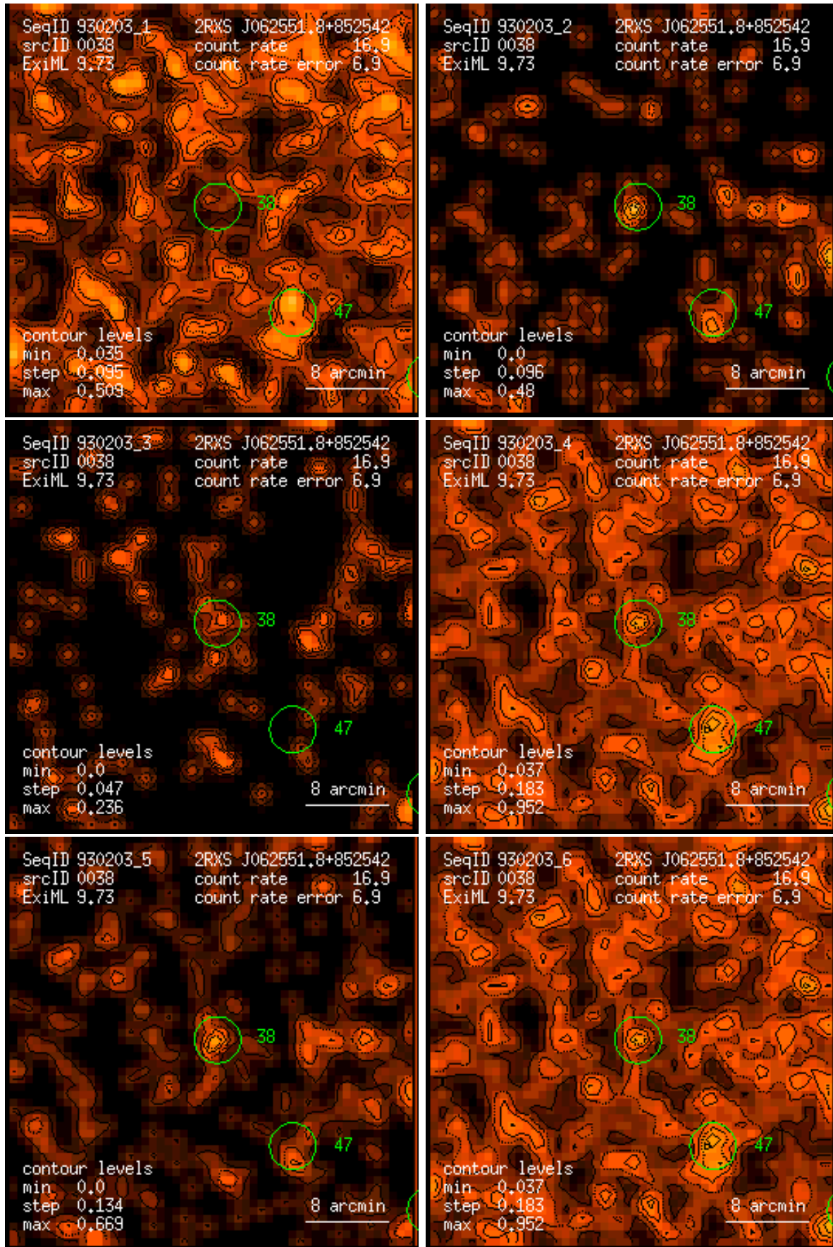
Figure 38: RASS 930203: detection 0038: band rate images, Gaussian filter: (1) PSPC channels 11 – 41, (2) 52 – 90, (3) 91 – 201, (4) 11 – 235, (5) 52 – 201, (6) 11 – 201. Broad band rates in counts/ks. Band rate contour levels in counts/ks/arcmin 2 .
