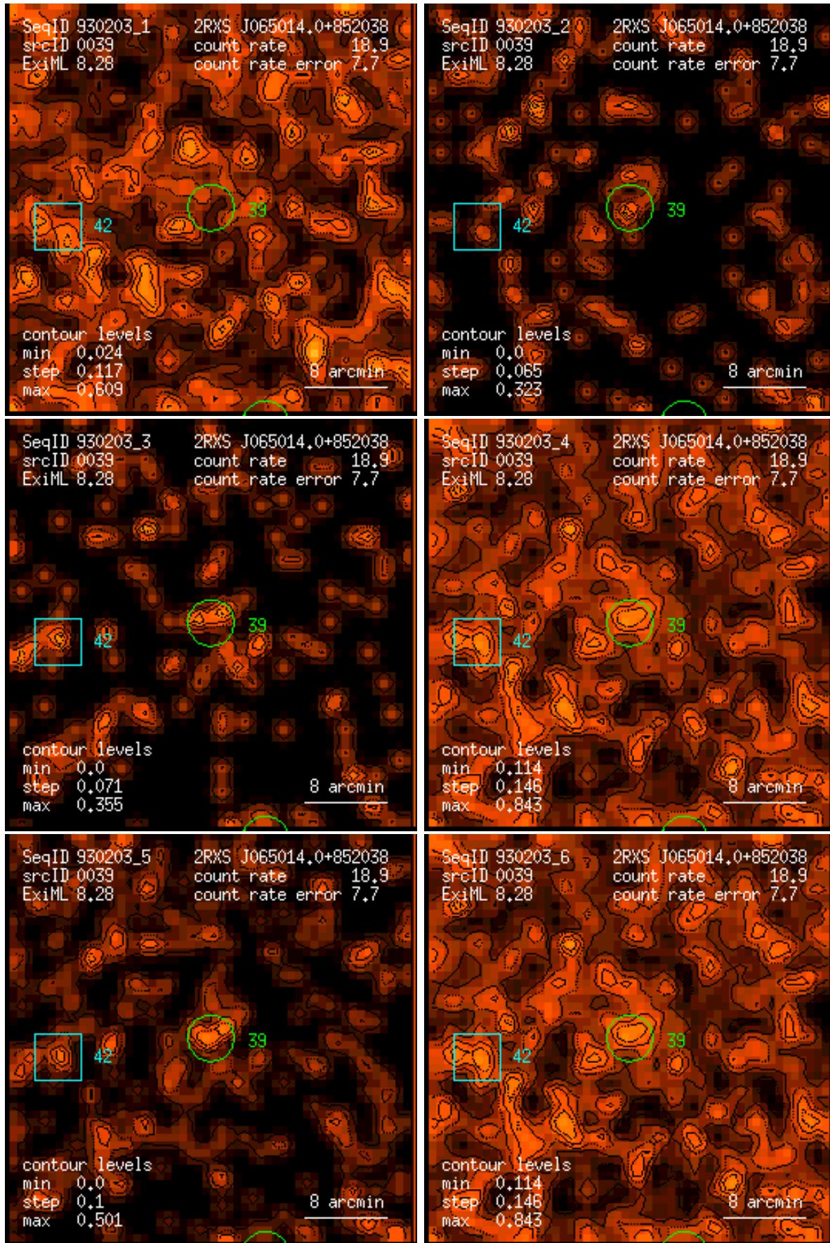
Figure 39: RASS 930203: detection 0039: band rate images, Gaussian filter: (1) PSPC channels 11 – 41, (2) 52 – 90, (3) 91 – 201, (4) 11 – 235, (5) 52 – 201, (6) 11 – 201. Broad band rates in counts/ks. Band rate contour levels in counts/ks/arcmin 2 .
