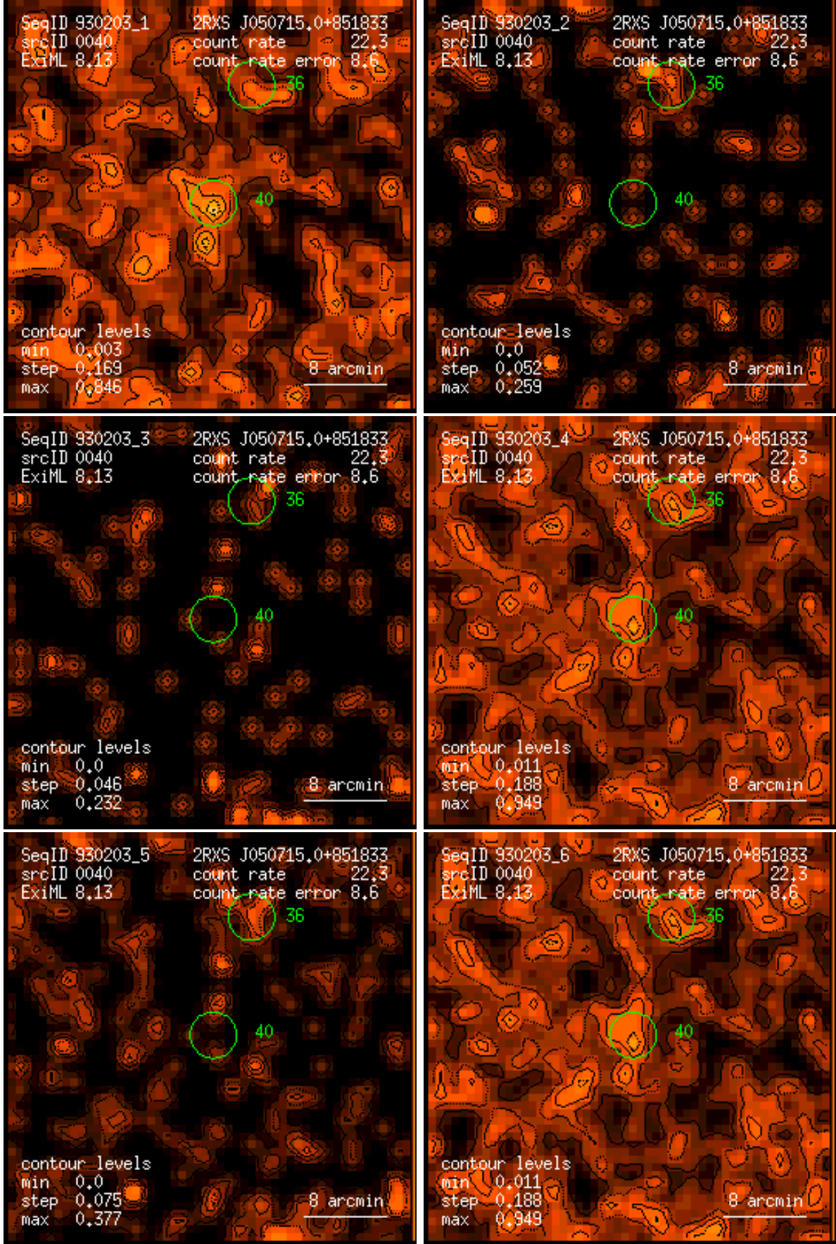
Figure 40: RASS 930203: detection 0040: band rate images, Gaussian filter: (1) PSPC channels 11 – 41, (2) 52 – 90, (3) 91 – 201, (4) 11 – 235, (5) 52 – 201, (6) 11 – 201. Broad band rates in counts/ks. Band rate contour levels in counts/ks/arcmin 2 .
