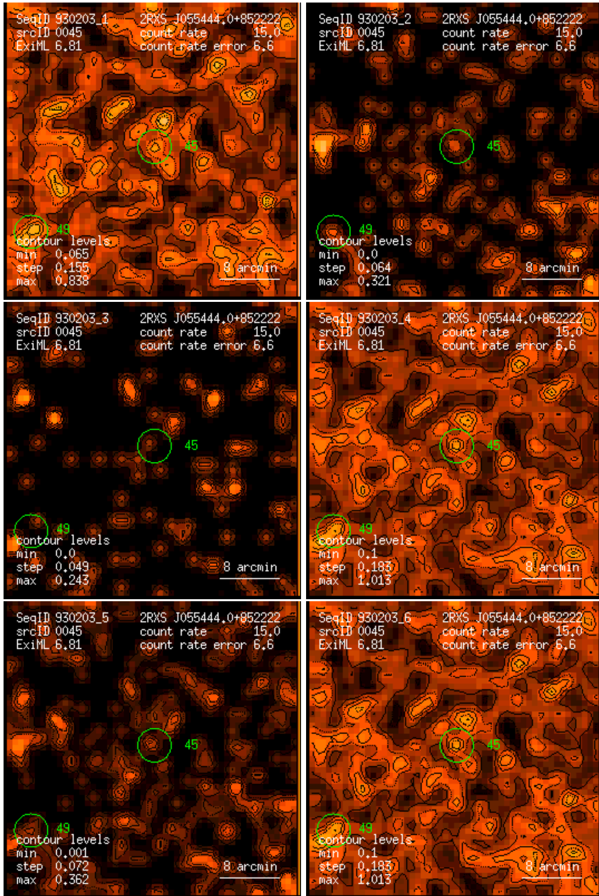
Figure 45: RASS 930203: detection 0045: band rate images, Gaussian filter: (1) PSPC channels 11 – 41, (2) 52 – 90, (3) 91 – 201, (4) 11 – 235, (5) 52 – 201, (6) 11 – 201. Broad band rates in counts/ks. Band rate contour levels in counts/ks/arcmin 2 .
