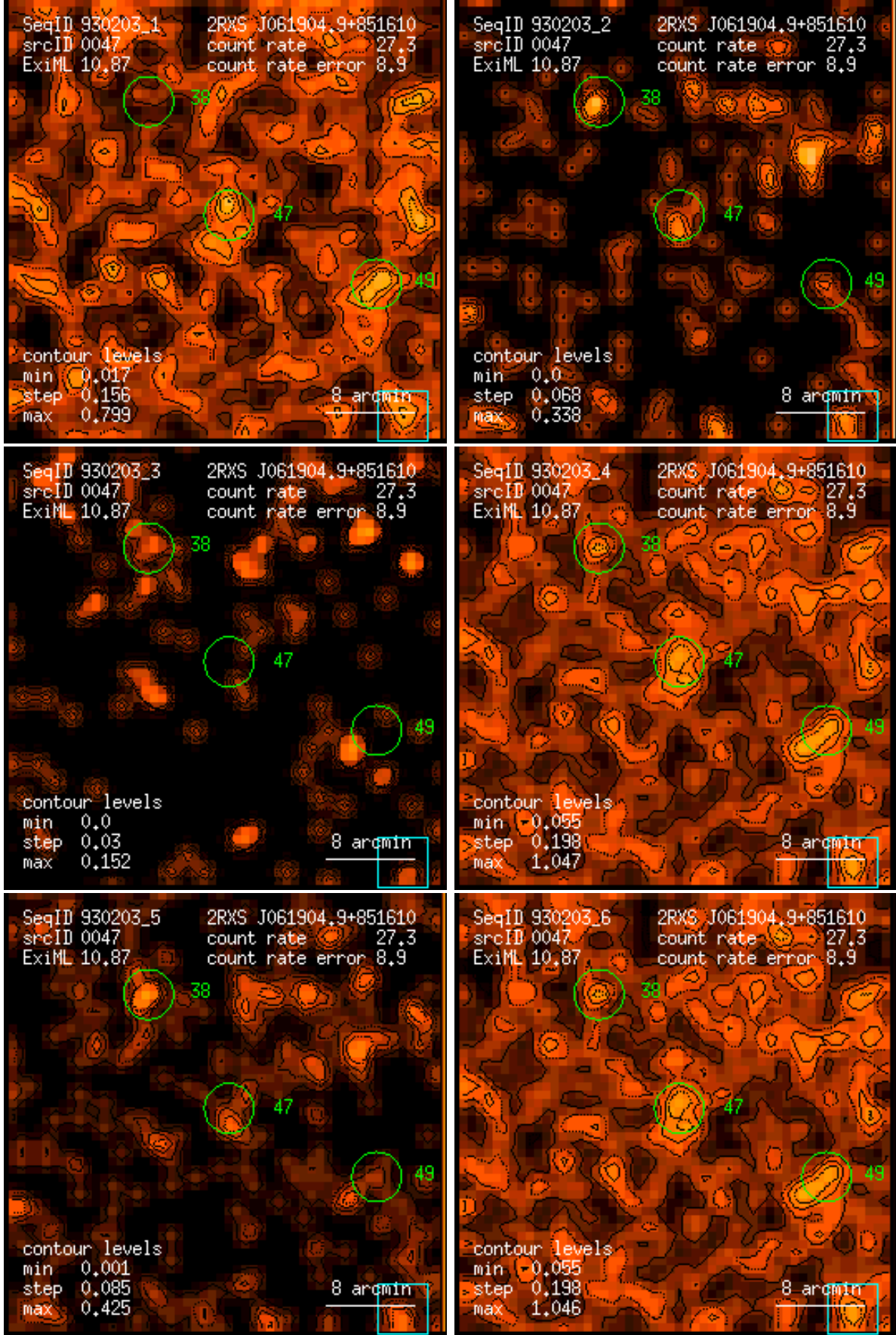
Figure 47: RASS 930203: detection 0047: band rate images, Gaussian filter: (1) PSPC channels 11 – 41, (2) 52 – 90, (3) 91 – 201, (4) 11 – 235, (5) 52 – 201, (6) 11 – 201. Broad band rates in counts/ks. Band rate contour levels in counts/ks/arcmin 2 .
