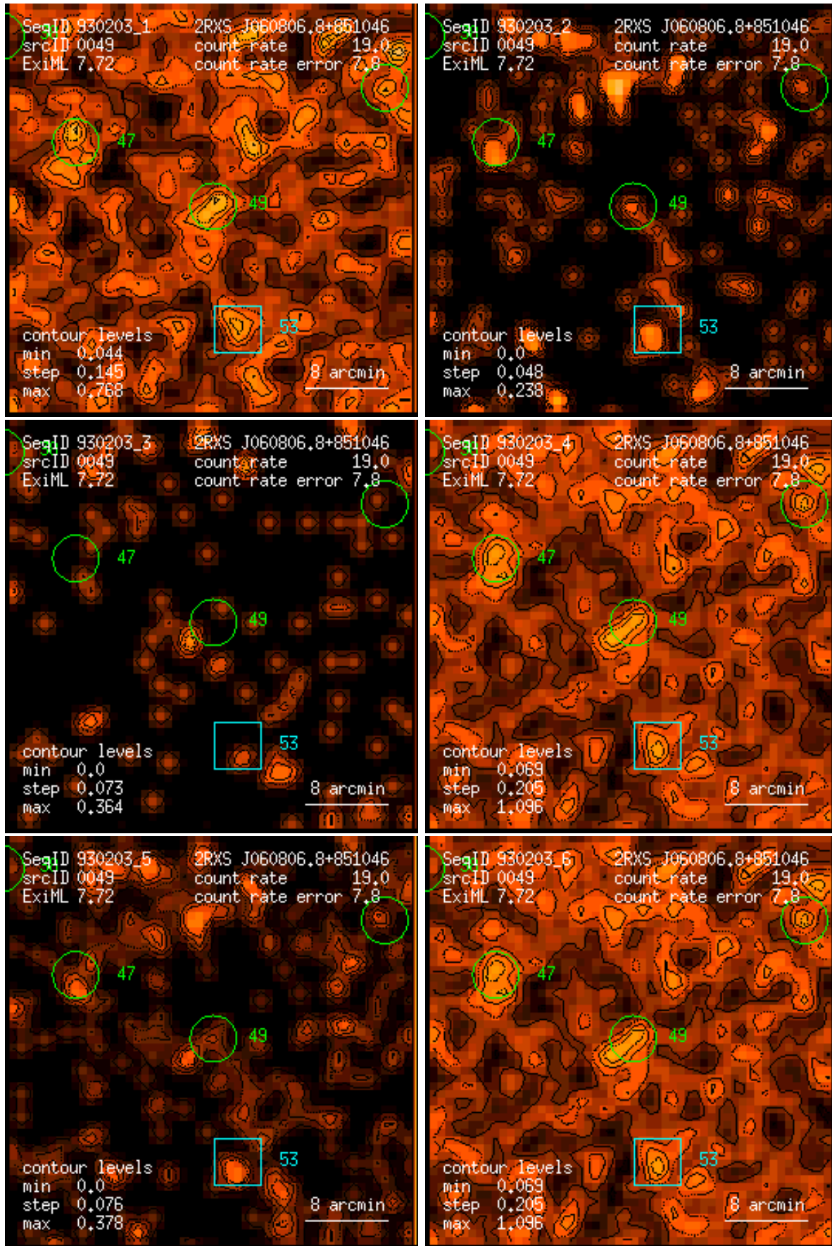
Figure 49: RASS 930203: detection 0049: band rate images, Gaussian filter: (1) PSPC channels 11 – 41, (2) 52 – 90, (3) 91 – 201, (4) 11 – 235, (5) 52 – 201, (6) 11 – 201. Broad band rates in counts/ks. Band rate contour levels in counts/ks/arcmin 2 .
