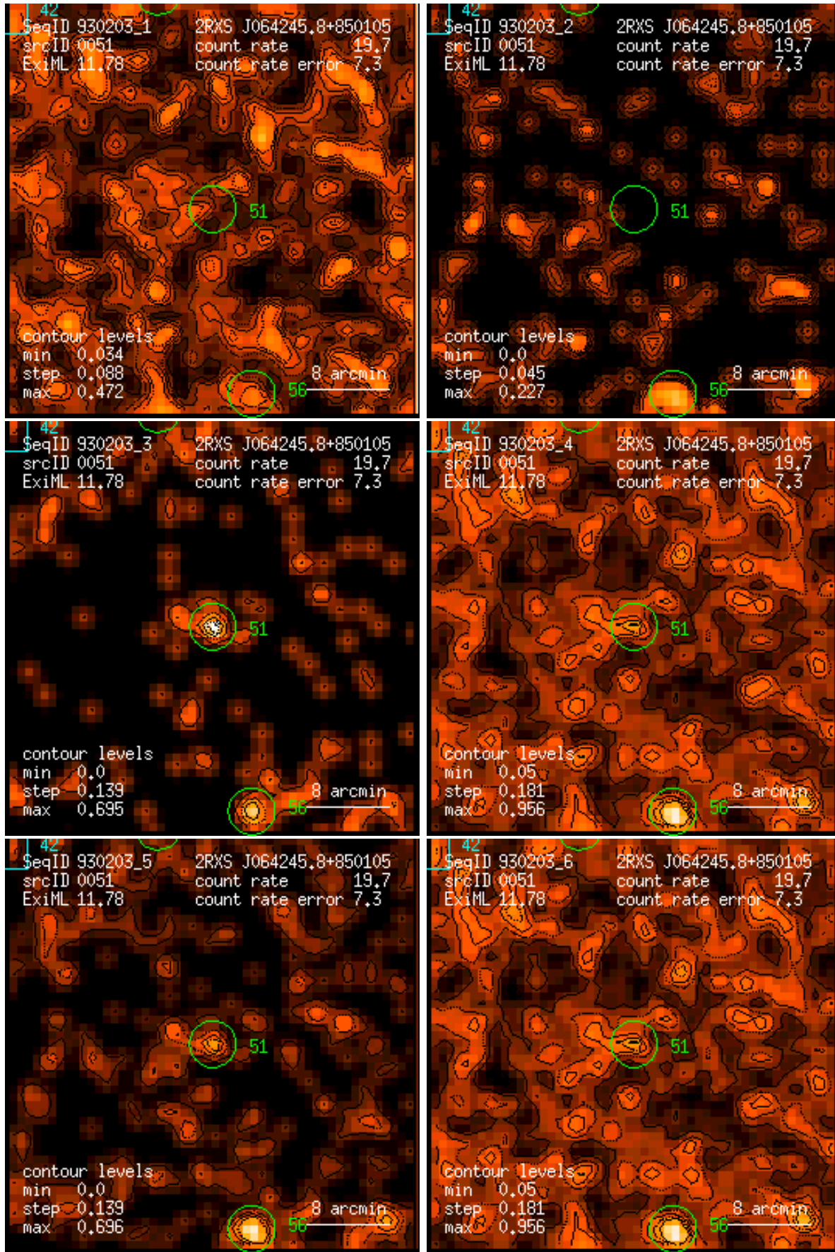
Figure 51: RASS 930203: detection 0051: band rate images, Gaussian filter: (1) PSPC channels 11 – 41, (2) 52 – 90, (3) 91 – 201, (4) 11 – 235, (5) 52 – 201, (6) 11 – 201. Broad band rates in counts/ks. Band rate contour levels in counts/ks/arcmin 2 .
