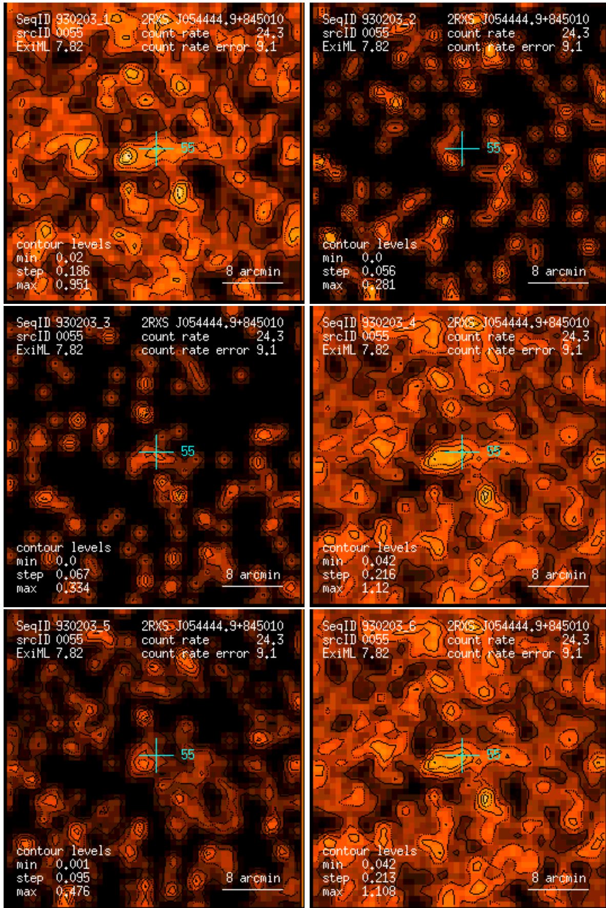
Figure 55: RASS 930203: detection 0055: band rate images, Gaussian filter: (1) PSPC channels 11 – 41, (2) 52 – 90, (3) 91 – 201, (4) 11 – 235, (5) 52 – 201, (6) 11 – 201. Broad band rates in counts/ks. Band rate contour levels in counts/ks/arcmin 2 .
