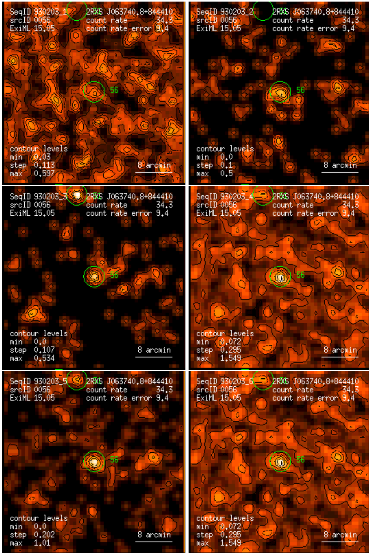
Figure 56: RASS 930203: detection 0056: band rate images, Gaussian filter: (1) PSPC channels 11 – 41, (2) 52 – 90, (3) 91 – 201, (4) 11 – 235, (5) 52 – 201, (6) 11 – 201. Broad band rates in counts/ks. Band rate contour levels in counts/ks/arcmin 2 .
