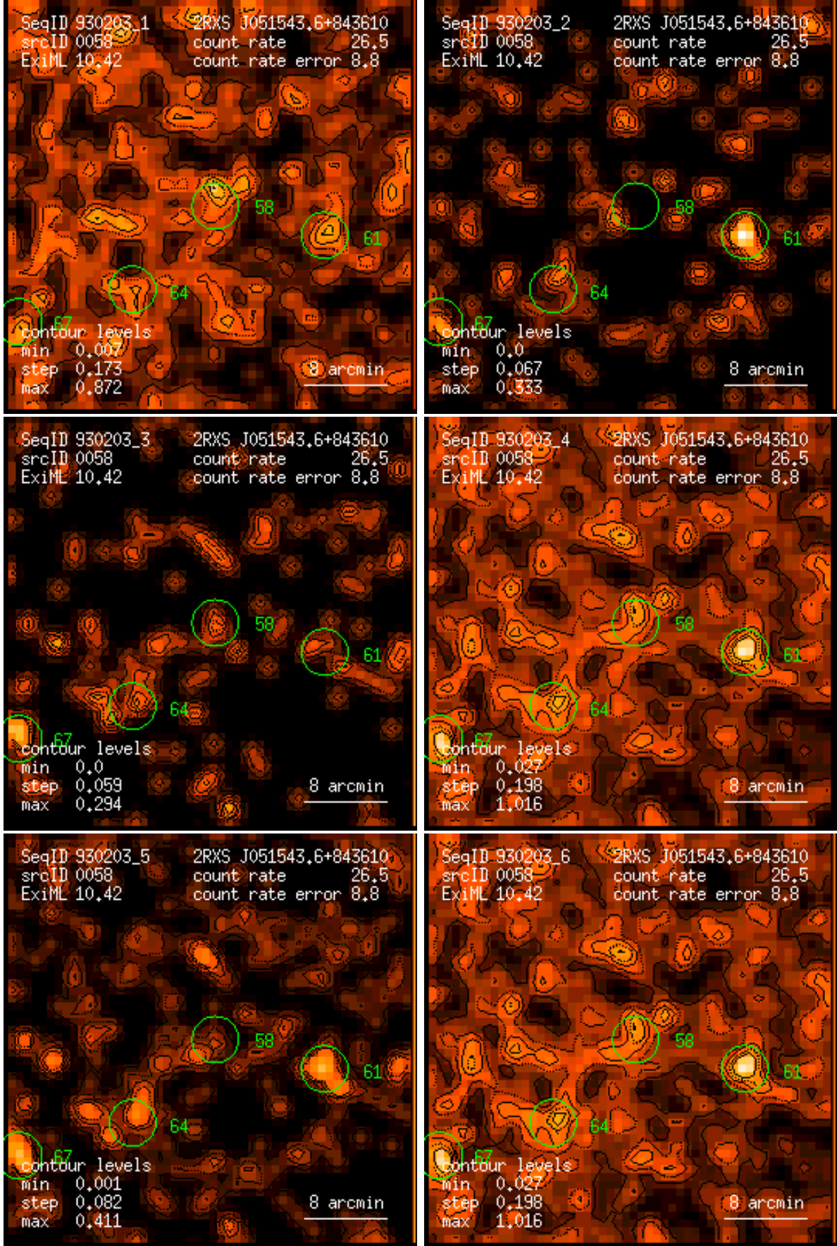
Figure 58: RASS 930203: detection 0058: band rate images, Gaussian filter: (1) PSPC channels 11 – 41, (2) 52 – 90, (3) 91 – 201, (4) 11 – 235, (5) 52 – 201, (6) 11 – 201. Broad band rates in counts/ks. Band rate contour levels in counts/ks/arcmin 2 .
