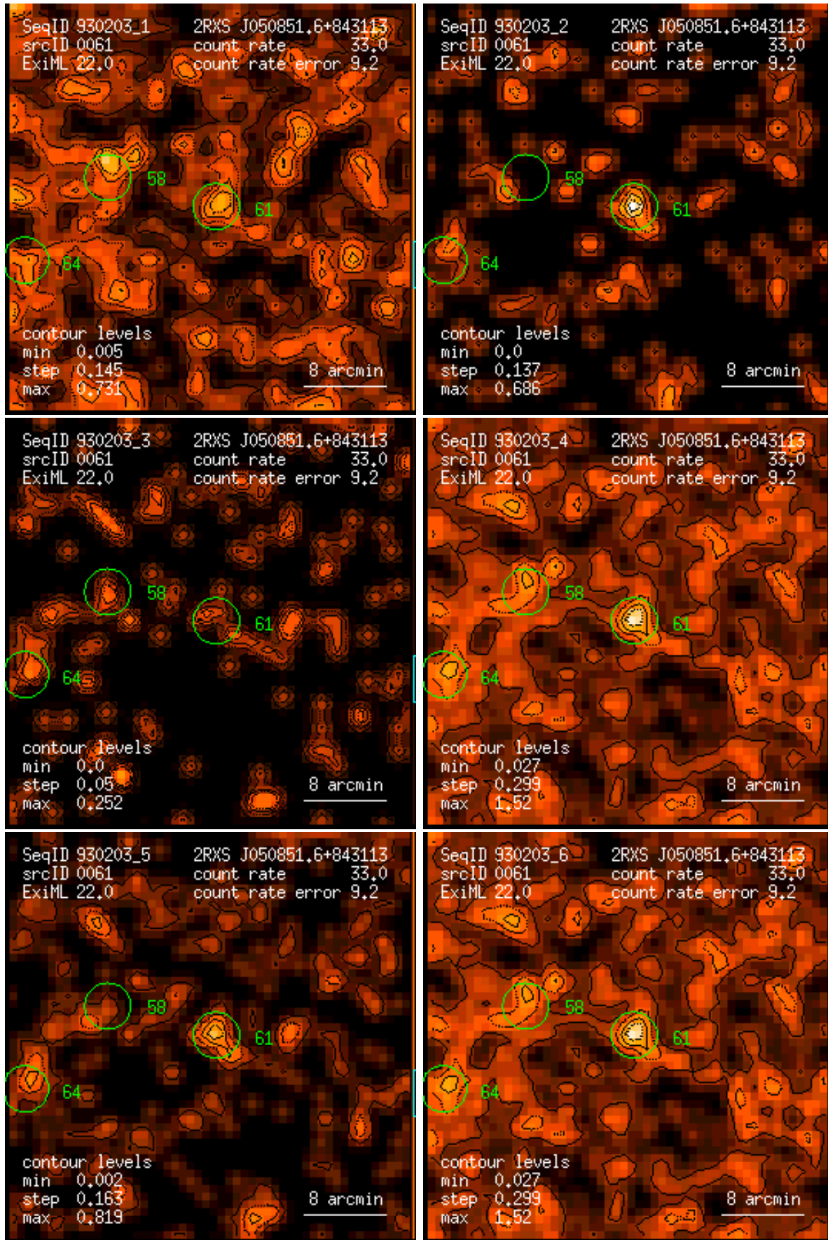
Figure 61: RASS 930203: detection 0061: band rate images, Gaussian filter: (1) PSPC channels 11 – 41, (2) 52 – 90, (3) 91 – 201, (4) 11 – 235, (5) 52 – 201, (6) 11 – 201. Broad band rates in counts/ks. Band rate contour levels in counts/ks/arcmin 2 .
