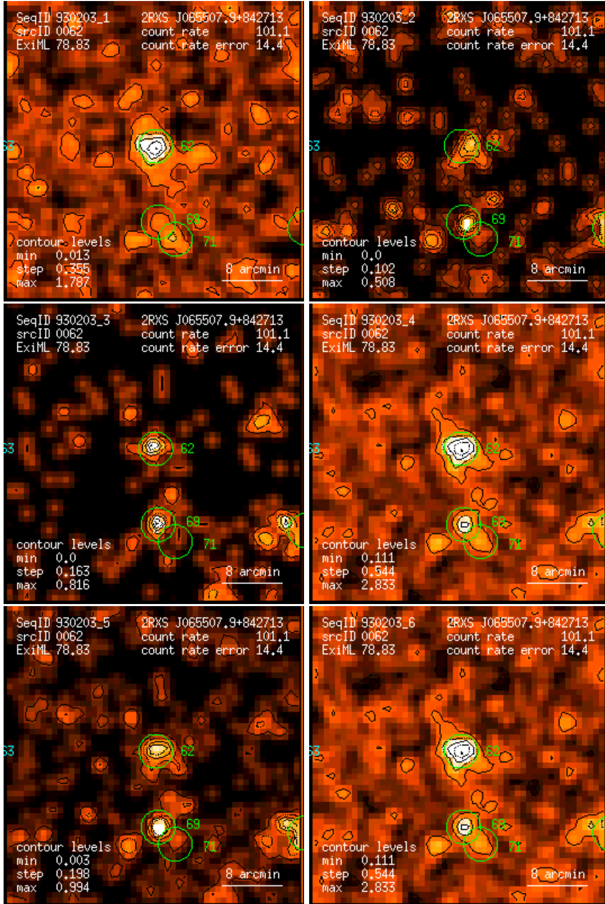
Figure 62: RASS 930203: detection 0062: band rate images, Gaussian filter: (1) PSPC channels 11 – 41, (2) 52 – 90, (3) 91 – 201, (4) 11 – 235, (5) 52 – 201, (6) 11 – 201. Broad band rates in counts/ks. Band rate contour levels in counts/ks/arcmin 2 .
