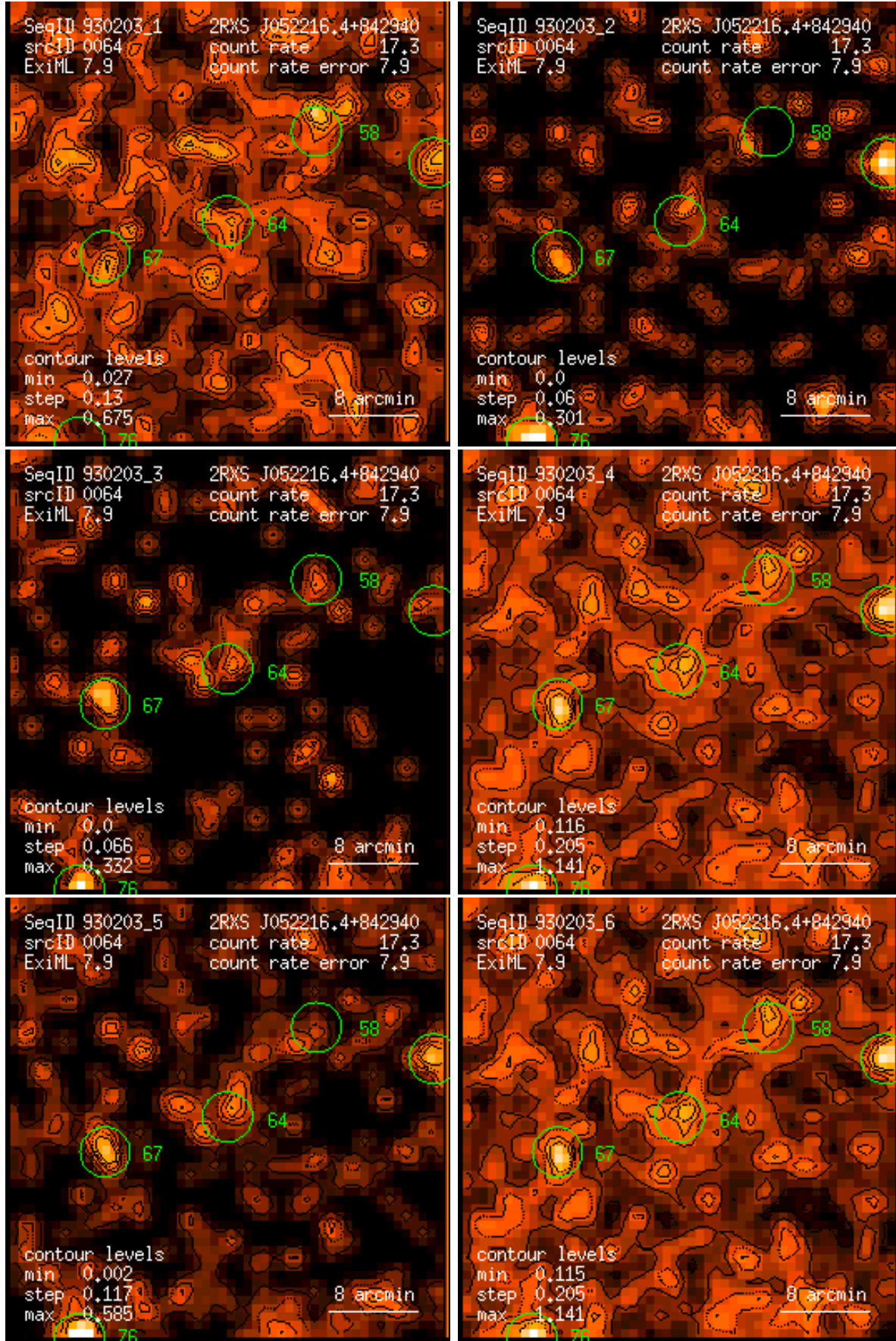
Figure 64: RASS 930203: detection 0064: band rate images, Gaussian filter: (1) PSPC channels 11 – 41, (2) 52 – 90, (3) 91 – 201, (4) 11 – 235, (5) 52 – 201, (6) 11 – 201. Broad band rates in counts/ks. Band rate contour levels in counts/ks/arcmin 2 .
