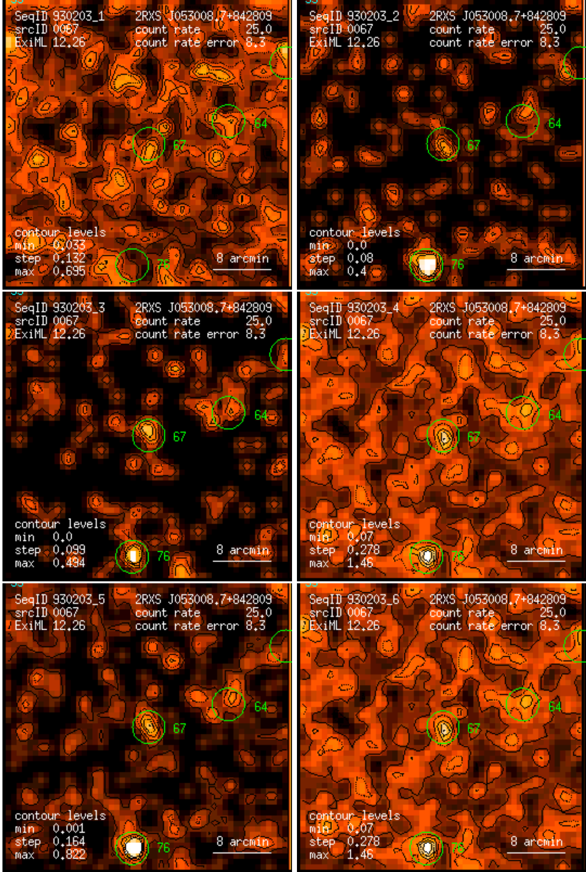
Figure 67: RASS 930203: detection 0067: band rate images, Gaussian filter: (1) PSPC channels 11 – 41, (2) 52 – 90, (3) 91 – 201, (4) 11 – 235, (5) 52 – 201, (6) 11 – 201. Broad band rates in counts/ks. Band rate contour levels in counts/ks/arcmin 2 .
