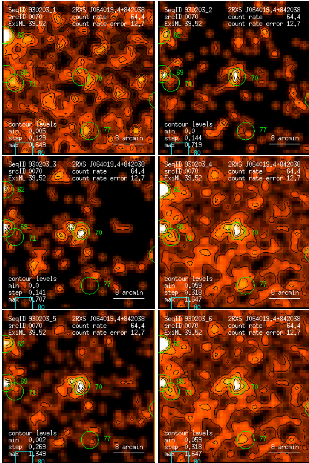
Figure 70: RASS 930203: detection 0070: band rate images, Gaussian filter: (1) PSPC channels 11 – 41, (2) 52 – 90, (3) 91 – 201, (4) 11 – 235, (5) 52 – 201, (6) 11 – 201. Broad band rates in counts/ks. Band rate contour levels in counts/ks/arcmin 2 .
