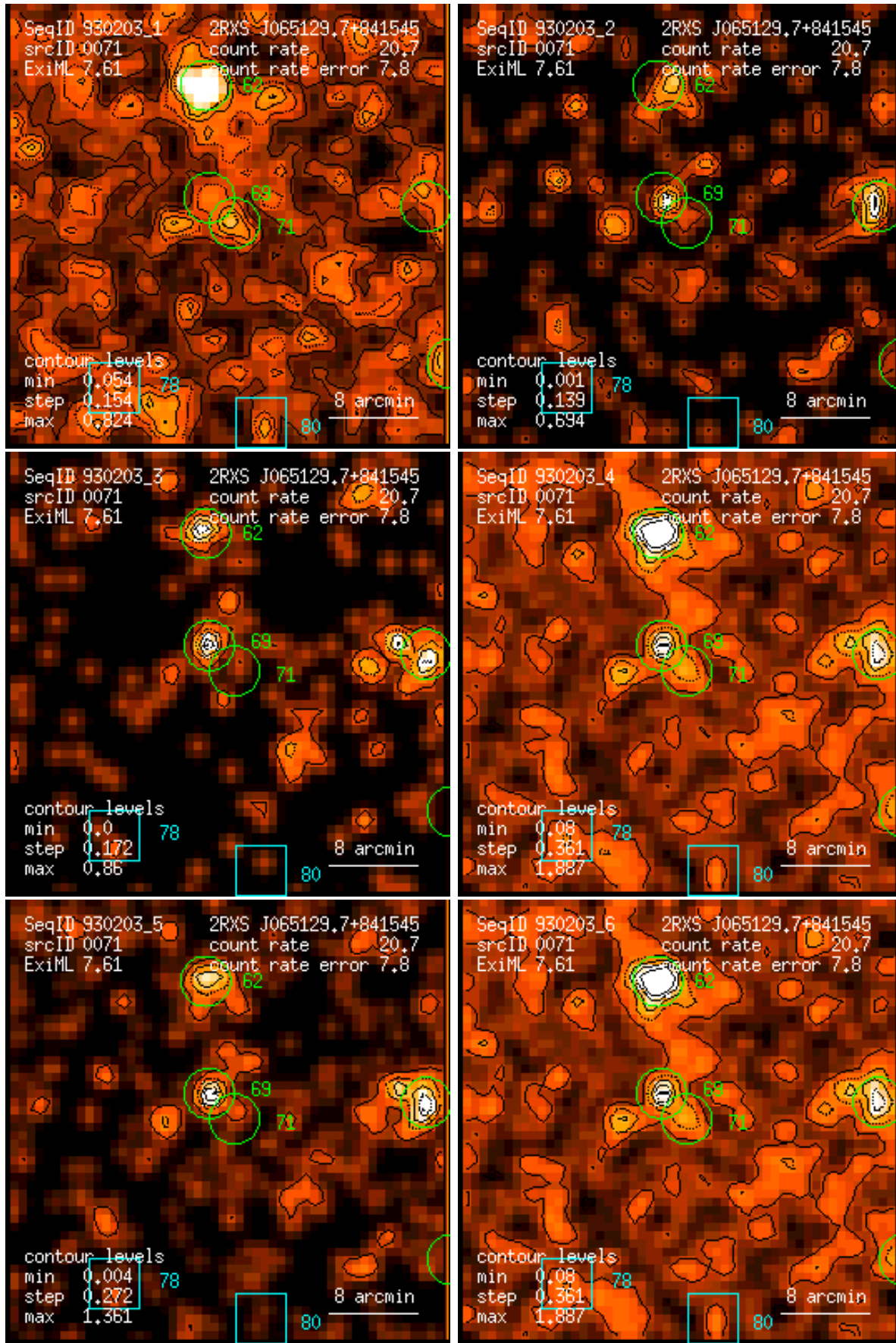
Figure 71: RASS 930203: detection 0071: band rate images, Gaussian filter: (1) PSPC channels 11 – 41, (2) 52 – 90, (3) 91 – 201, (4) 11 – 235, (5) 52 – 201, (6) 11 – 201. Broad band rates in counts/ks. Band rate contour levels in counts/ks/arcmin 2 .
