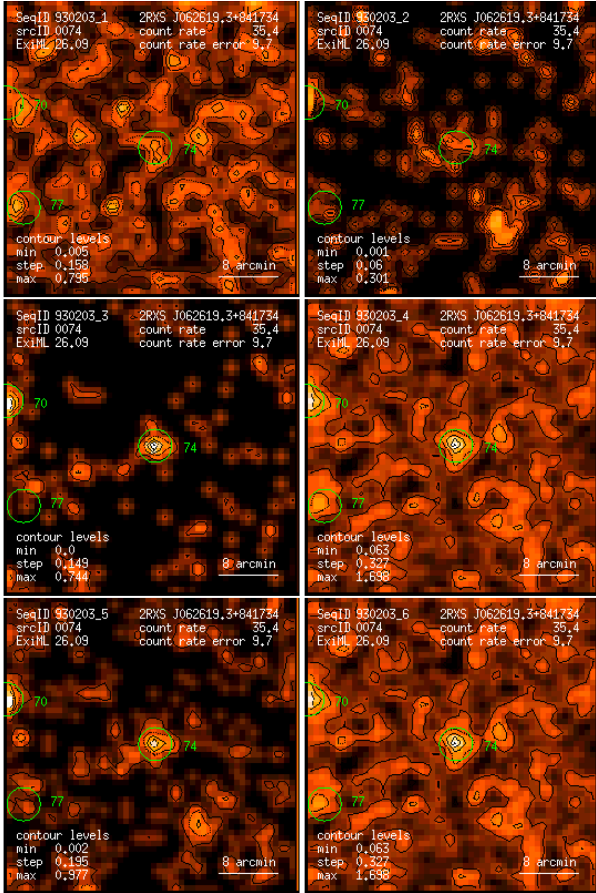
Figure 74: RASS 930203: detection 0074: band rate images, Gaussian filter: (1) PSPC channels 11 – 41, (2) 52 – 90, (3) 91 – 201, (4) 11 – 235, (5) 52 – 201, (6) 11 – 201. Broad band rates in counts/ks. Band rate contour levels in counts/ks/arcmin 2 .
