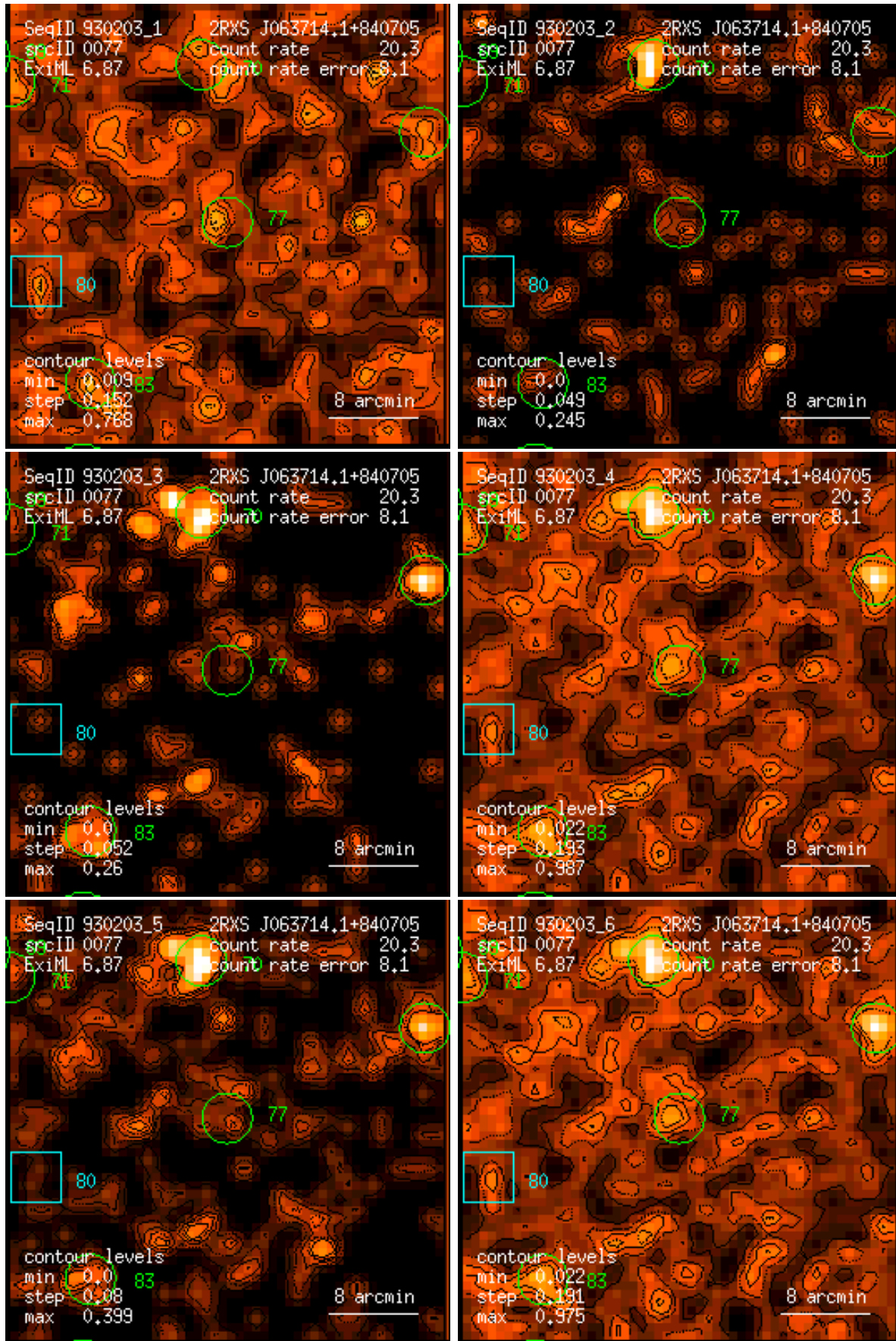
Figure 77: RASS 930203: detection 0077: band rate images, Gaussian filter: (1) PSPC channels 11 – 41, (2) 52 – 90, (3) 91 – 201, (4) 11 – 235, (5) 52 – 201, (6) 11 – 201. Broad band rates in counts/ks. Band rate contour levels in counts/ks/arcmin 2 .
