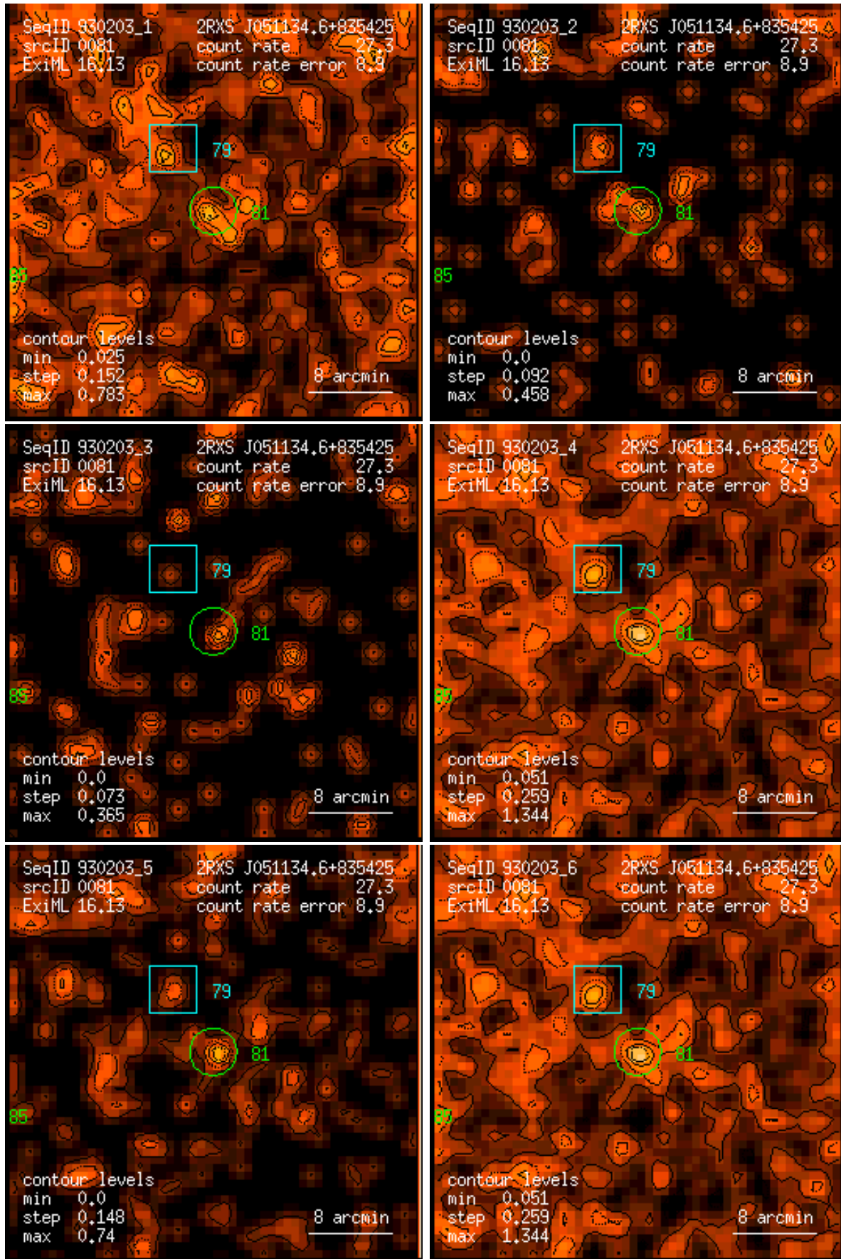
Figure 81: RASS 930203: detection 0081: band rate images, Gaussian filter: (1) PSPC channels 11 – 41, (2) 52 – 90, (3) 91 – 201, (4) 11 – 235, (5) 52 – 201, (6) 11 – 201. Broad band rates in counts/ks. Band rate contour levels in counts/ks/arcmin 2 .
