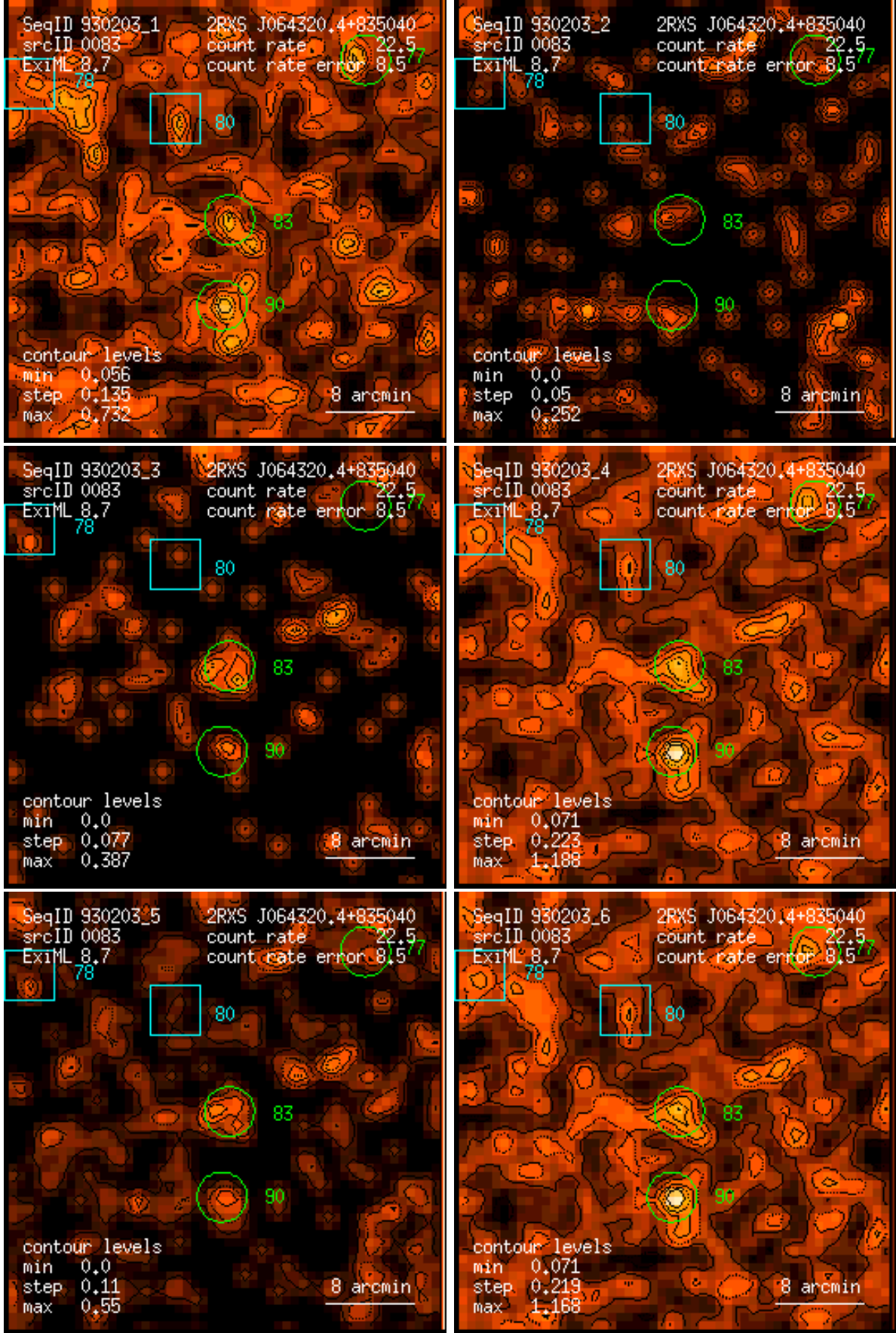
Figure 83: RASS 930203: detection 0083: band rate images, Gaussian filter: (1) PSPC channels 11 – 41, (2) 52 – 90, (3) 91 – 201, (4) 11 – 235, (5) 52 – 201, (6) 11 – 201. Broad band rates in counts/ks. Band rate contour levels in counts/ks/arcmin 2 .
