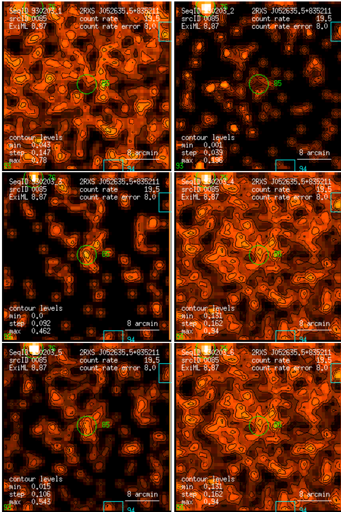
Figure 85: RASS 930203: detection 0085: band rate images, Gaussian filter: (1) PSPC channels 11 – 41, (2) 52 – 90, (3) 91 – 201, (4) 11 – 235, (5) 52 – 201, (6) 11 – 201. Broad band rates in counts/ks. Band rate contour levels in counts/ks/arcmin 2 .
