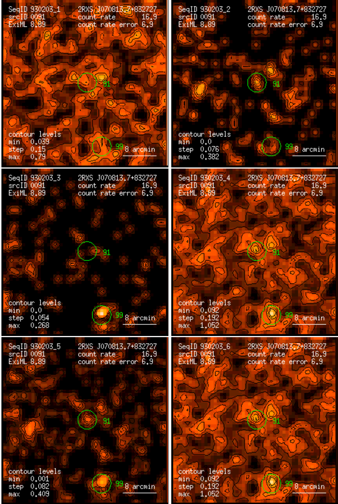
Figure 91: RASS 930203: detection 0091: band rate images, Gaussian filter: (1) PSPC channels 11 – 41, (2) 52 – 90, (3) 91 – 201, (4) 11 – 235, (5) 52 – 201, (6) 11 – 201. Broad band rates in counts/ks. Band rate contour levels in counts/ks/arcmin 2 .
