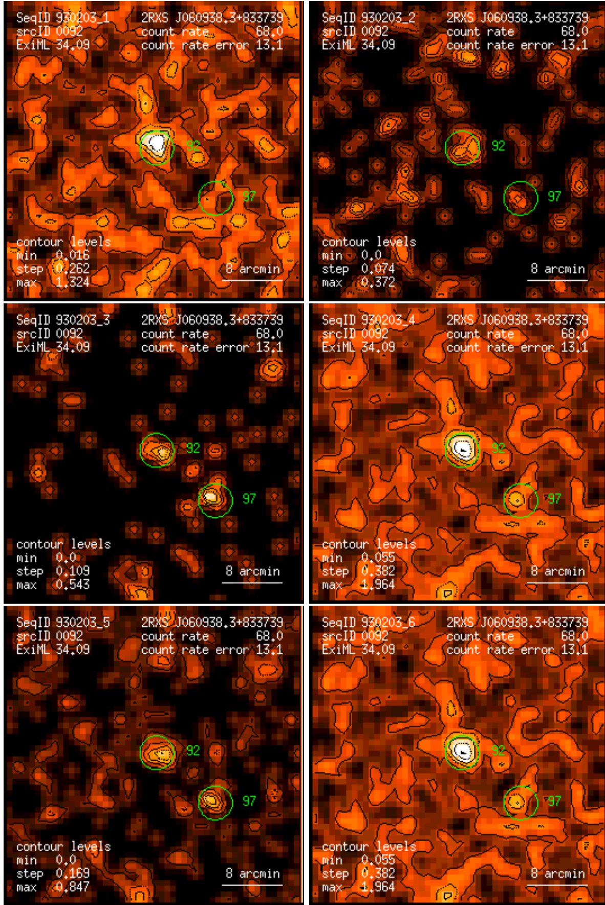
Figure 92: RASS 930203: detection 0092: band rate images, Gaussian filter: (1) PSPC channels 11 – 41, (2) 52 – 90, (3) 91 – 201, (4) 11 – 235, (5) 52 – 201, (6) 11 – 201. Broad band rates in counts/ks. Band rate contour levels in counts/ks/arcmin 2 .
