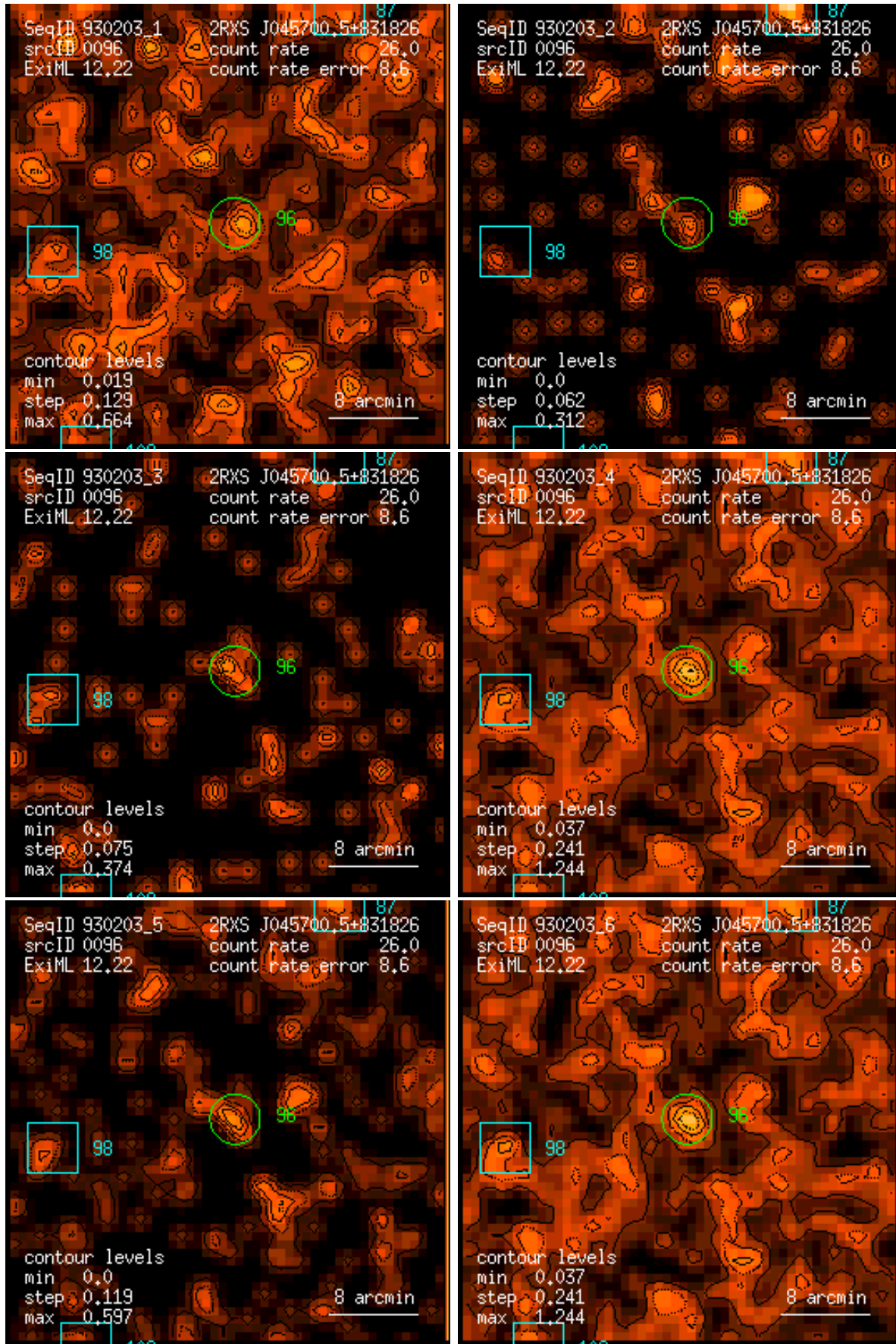
Figure 96: RASS 930203: detection 0096: band rate images, Gaussian filter: (1) PSPC channels 11 – 41, (2) 52 – 90, (3) 91 – 201, (4) 11 – 235, (5) 52 – 201, (6) 11 – 201. Broad band rates in counts/ks. Band rate contour levels in counts/ks/arcmin 2 .
