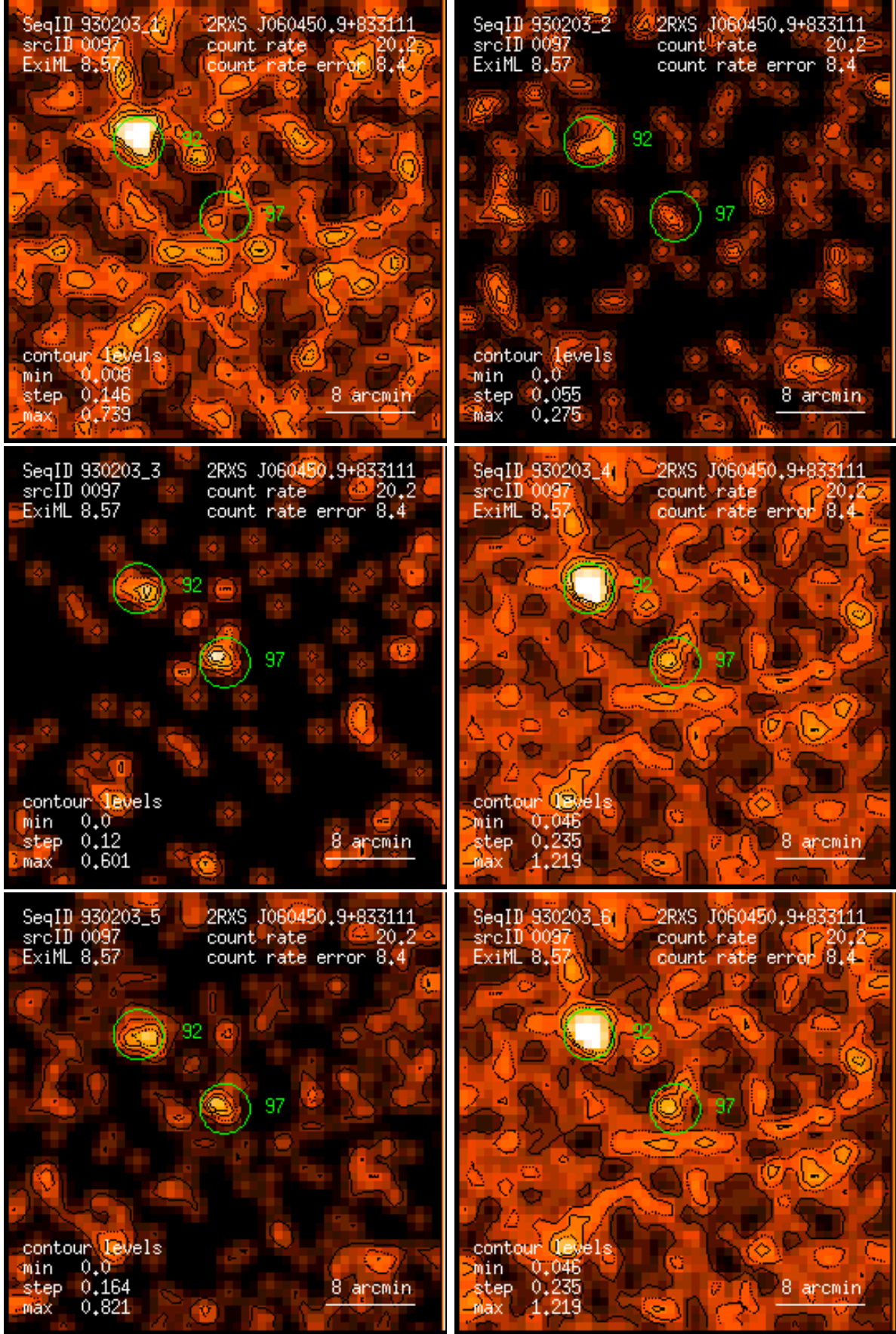
Figure 97: RASS 930203: detection 0097: band rate images, Gaussian filter: (1) PSPC channels 11 – 41, (2) 52 – 90, (3) 91 – 201, (4) 11 – 235, (5) 52 – 201, (6) 11 – 201. Broad band rates in counts/ks. Band rate contour levels in counts/ks/arcmin 2 .
