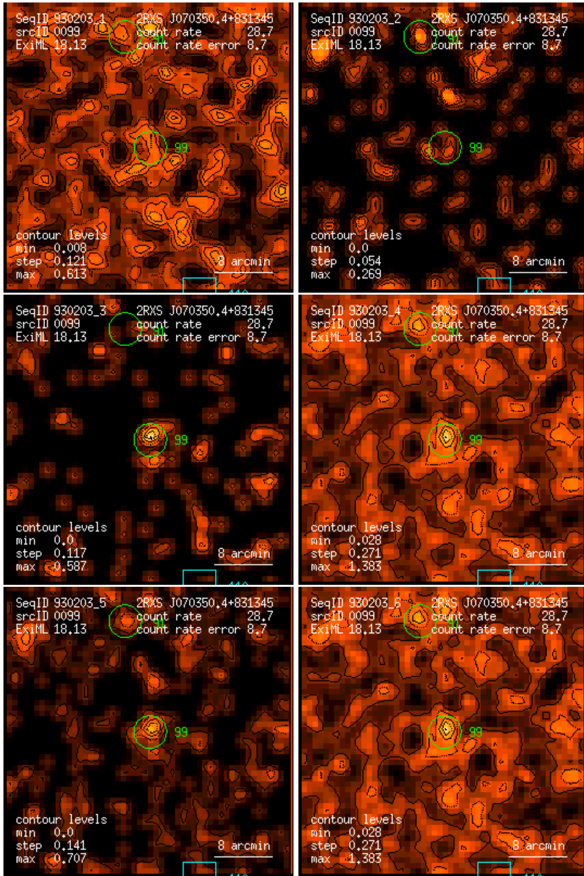
Figure 99: RASS 930203: detection 0099: band rate images, Gaussian filter: (1) PSPC channels 11 – 41, (2) 52 – 90, (3) 91 – 201, (4) 11 – 235, (5) 52 – 201, (6) 11 – 201. Broad band rates in counts/ks. Band rate contour levels in counts/ks/arcmin 2 .
