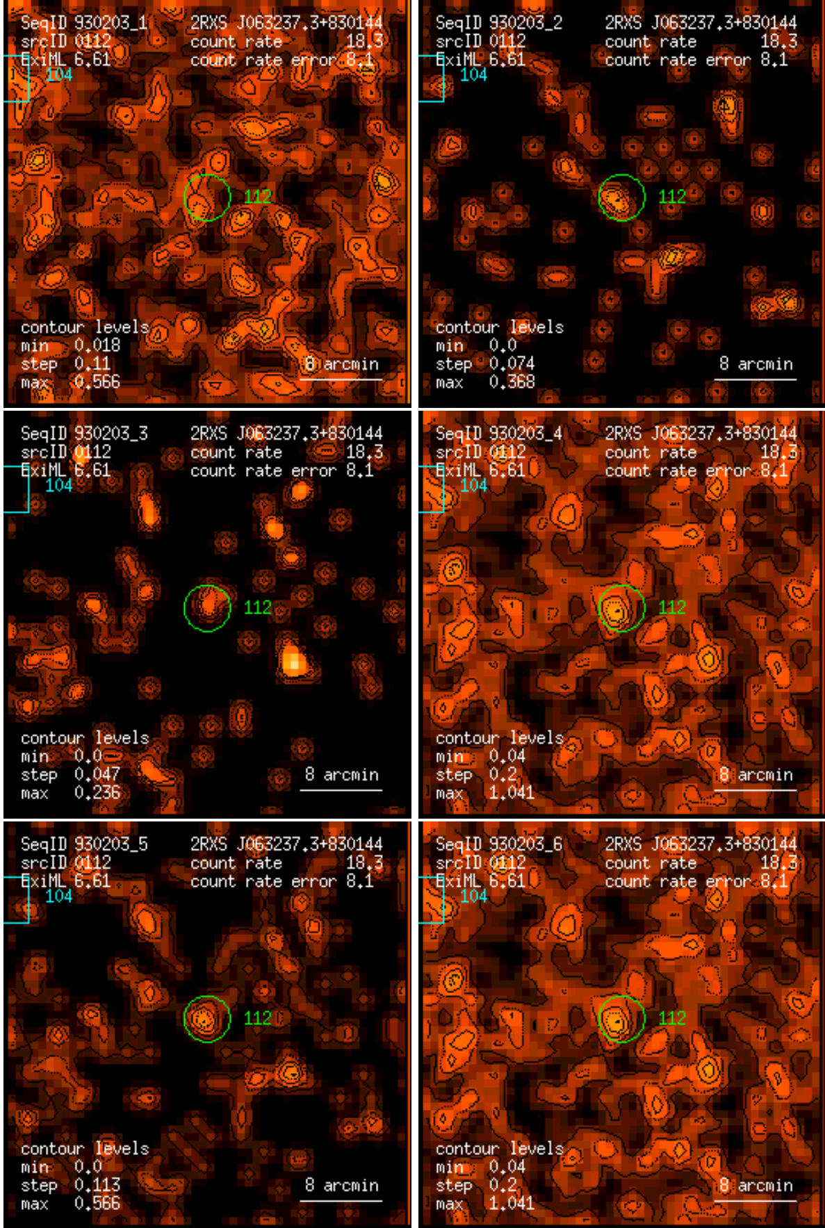
Figure 112: RASS 930203: detection 0112: band rate images, Gaussian filter: (1) PSPC channels 11 – 41, (2) 52 – 90, (3) 91 – 201, (4) 11 – 235, (5) 52 – 201, (6) 11 – 201. Broad band rates in counts/ks. Band rate contour levels in counts/ks/arcmin 2 .
