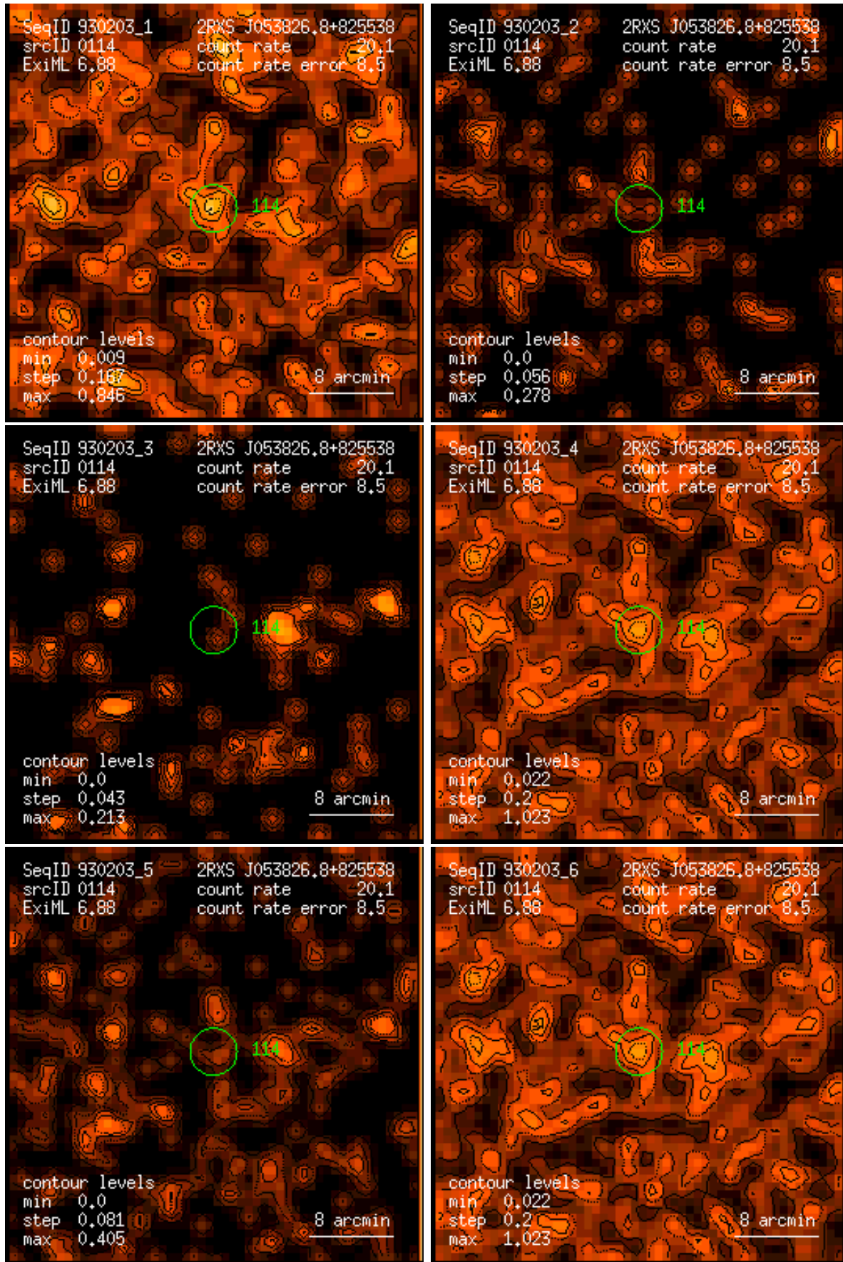
Figure 114: RASS 930203: detection 0114: band rate images, Gaussian filter: (1) PSPC channels 11 – 41, (2) 52 – 90, (3) 91 – 201, (4) 11 – 235, (5) 52 – 201, (6) 11 – 201. Broad band rates in counts/ks. Band rate contour levels in counts/ks/arcmin 2 .
