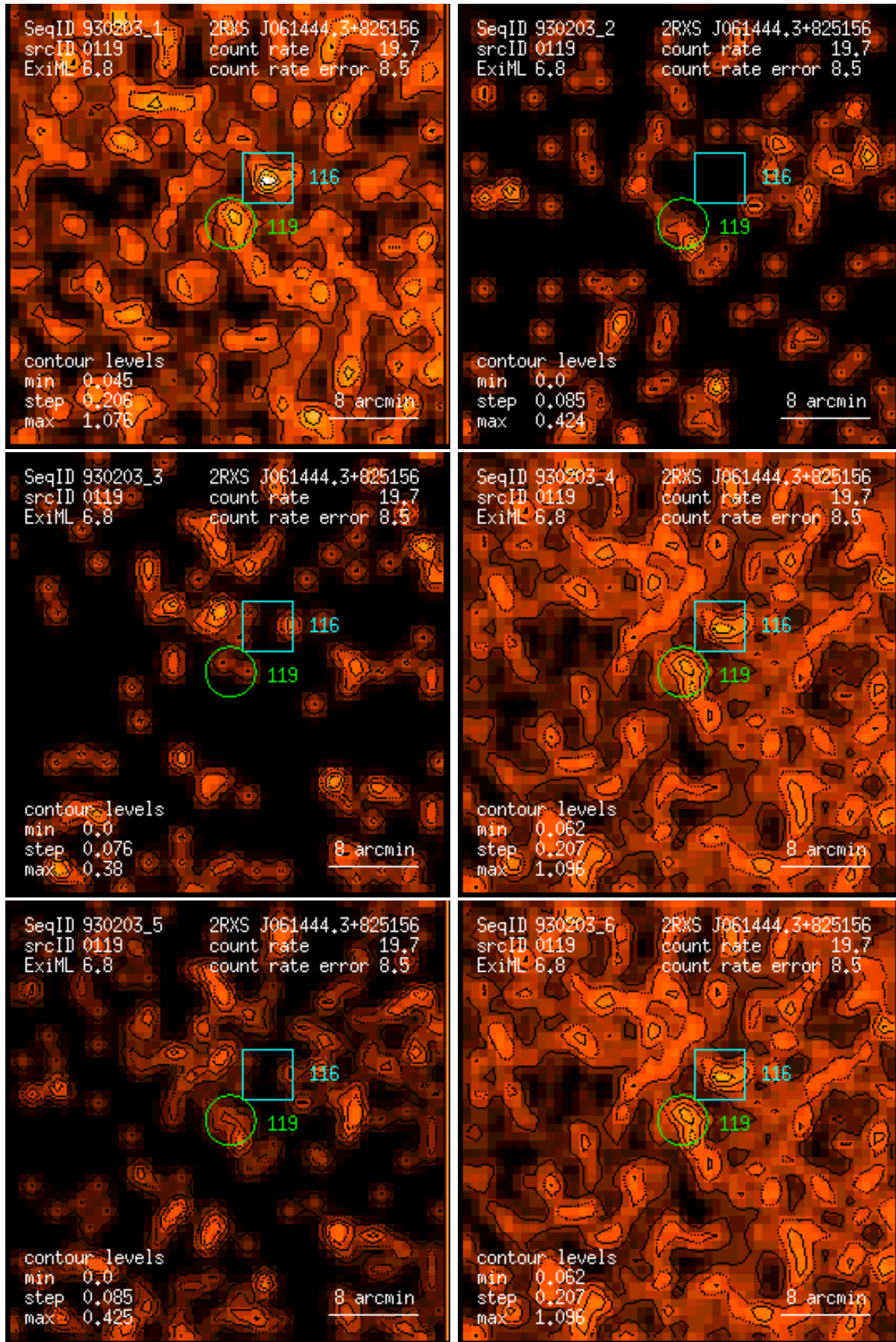
Figure 119: RASS 930203: detection 0119: band rate images, Gaussian filter: (1) PSPC channels 11 – 41, (2) 52 – 90, (3) 91 – 201, (4) 11 – 235, (5) 52 – 201, (6) 11 – 201. Broad band rates in counts/ks. Band rate contour levels in counts/ks/arcmin 2 .
