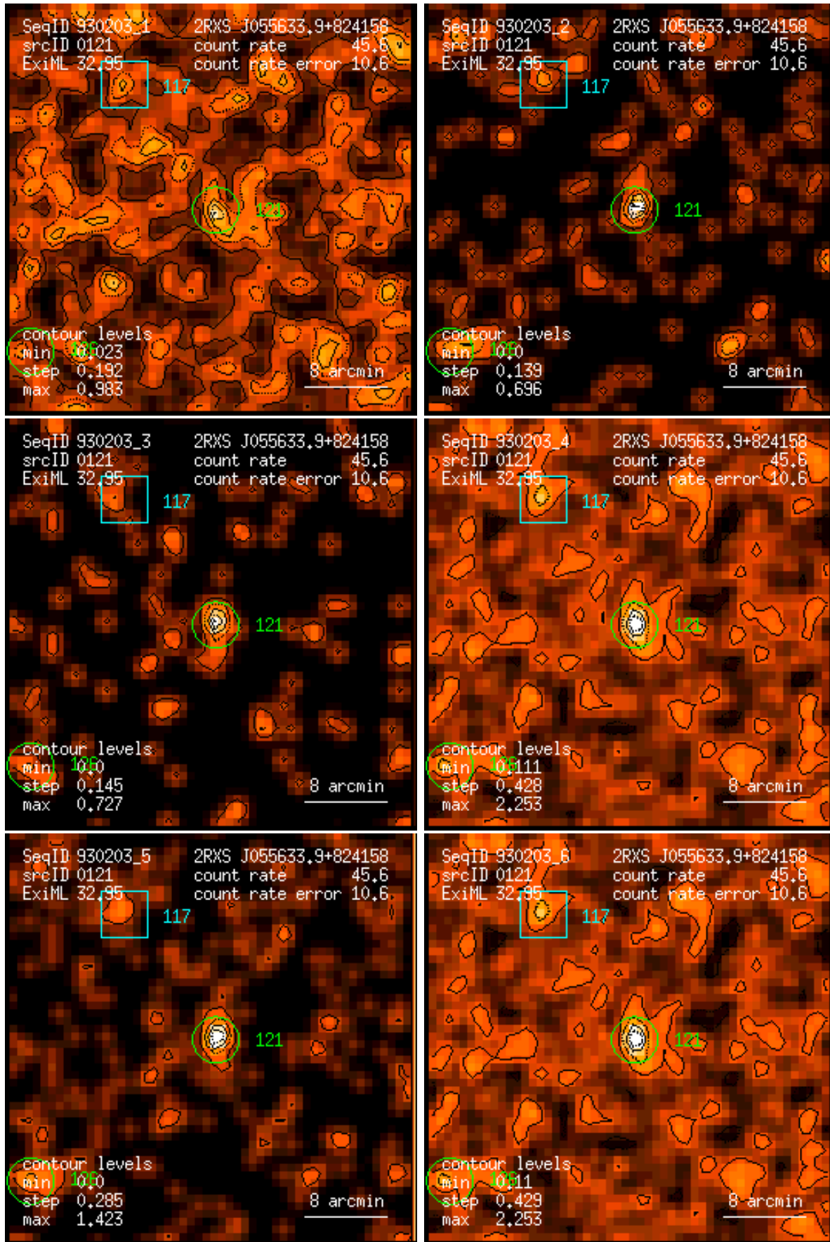
Figure 121: RASS 930203: detection 0121: band rate images, Gaussian filter: (1) PSPC channels 11 – 41, (2) 52 – 90, (3) 91 – 201, (4) 11 – 235, (5) 52 – 201, (6) 11 – 201. Broad band rates in counts/ks. Band rate contour levels in counts/ks/arcmin 2 .
