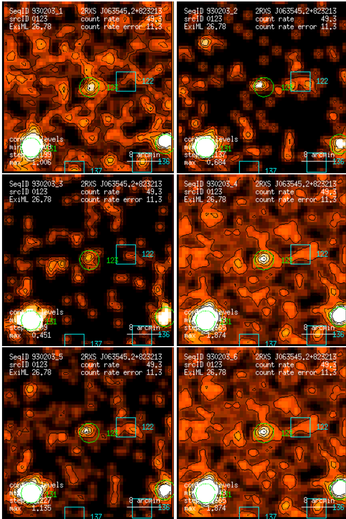
Figure 123: RASS 930203: detection 0123: band rate images, Gaussian filter: (1) PSPC channels 11 – 41, (2) 52 – 90, (3) 91 – 201, (4) 11 – 235, (5) 52 – 201, (6) 11 – 201. Broad band rates in counts/ks. Band rate contour levels in counts/ks/arcmin 2 .
