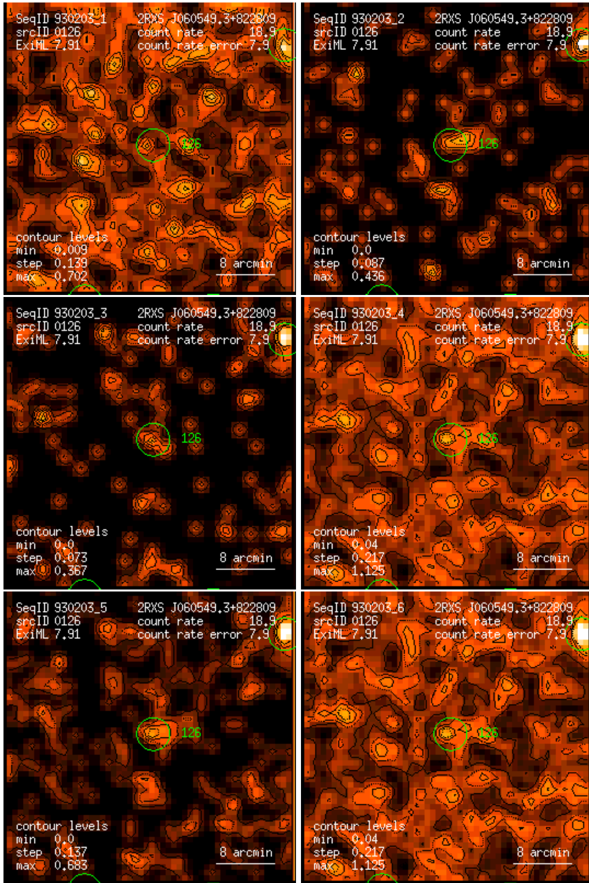
Figure 126: RASS 930203: detection 0126: band rate images, Gaussian filter: (1) PSPC channels 11 – 41, (2) 52 – 90, (3) 91 – 201, (4) 11 – 235, (5) 52 – 201, (6) 11 – 201. Broad band rates in counts/ks. Band rate contour levels in counts/ks/arcmin 2 .
