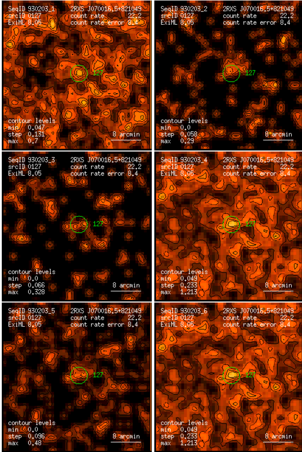
Figure 127: RASS 930203: detection 0127: band rate images, Gaussian filter: (1) PSPC channels 11 – 41, (2) 52 – 90, (3) 91 – 201, (4) 11 – 235, (5) 52 – 201, (6) 11 – 201. Broad band rates in counts/ks. Band rate contour levels in counts/ks/arcmin 2 .
