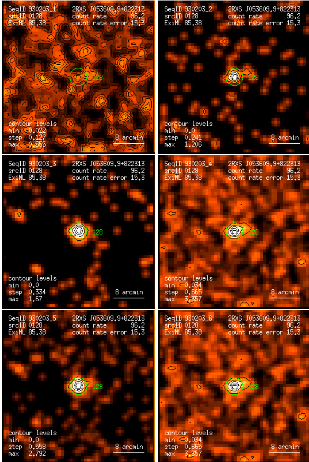
Figure 128: RASS 930203: detection 0128: band rate images, Gaussian filter: (1) PSPC channels 11 – 41, (2) 52 – 90, (3) 91 – 201, (4) 11 – 235, (5) 52 – 201, (6) 11 – 201. Broad band rates in counts/ks. Band rate contour levels in counts/ks/arcmin 2 .
