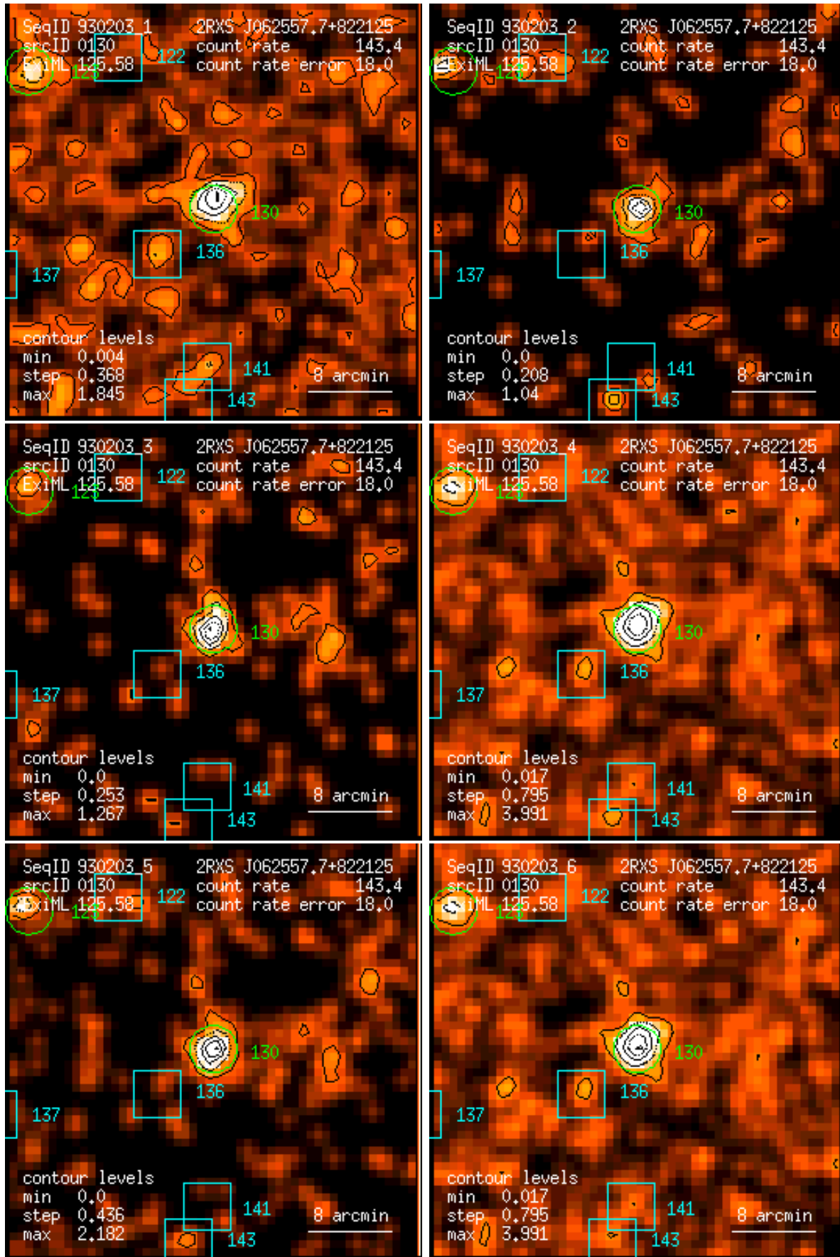
Figure 130: RASS 930203: detection 0130: band rate images, Gaussian filter: (1) PSPC channels 11 – 41, (2) 52 – 90, (3) 91 – 201, (4) 11 – 235, (5) 52 – 201, (6) 11 – 201. Broad band rates in counts/ks. Band rate contour levels in counts/ks/arcmin 2 .
