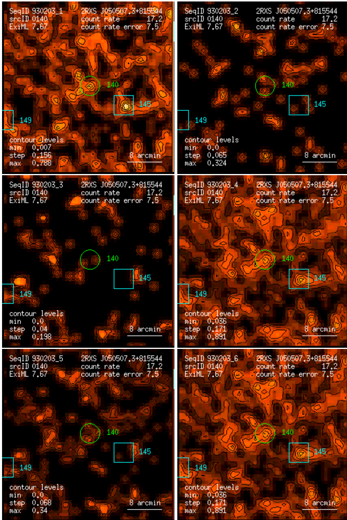
Figure 140: RASS 930203: detection 0140: band rate images, Gaussian filter: (1) PSPC channels 11 – 41, (2) 52 – 90, (3) 91 – 201, (4) 11 – 235, (5) 52 – 201, (6) 11 – 201. Broad band rates in counts/ks. Band rate contour levels in counts/ks/arcmin 2 .
