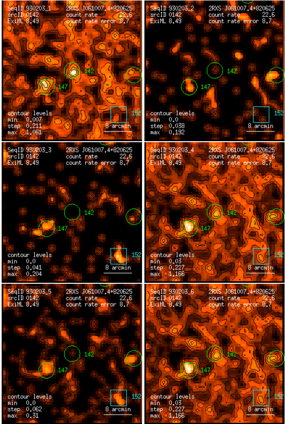
Figure 142: RASS 930203: detection 0142: band rate images, Gaussian filter: (1) PSPC channels 11 – 41, (2) 52 – 90, (3) 91 – 201, (4) 11 – 235, (5) 52 – 201, (6) 11 – 201. Broad band rates in counts/ks. Band rate contour levels in counts/ks/arcmin 2 .
