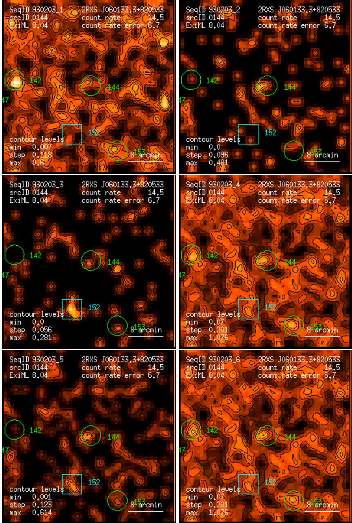
Figure 144: RASS 930203: detection 0144: band rate images, Gaussian filter: (1) PSPC channels 11 – 41, (2) 52 – 90, (3) 91 – 201, (4) 11 – 235, (5) 52 – 201, (6) 11 – 201. Broad band rates in counts/ks. Band rate contour levels in counts/ks/arcmin 2 .
