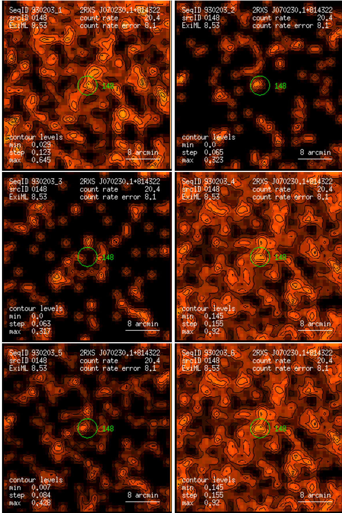
Figure 148: RASS 930203: detection 0148: band rate images, Gaussian filter: (1) PSPC channels 11 – 41, (2) 52 – 90, (3) 91 – 201, (4) 11 – 235, (5) 52 – 201, (6) 11 – 201. Broad band rates in counts/ks. Band rate contour levels in counts/ks/arcmin 2 .
