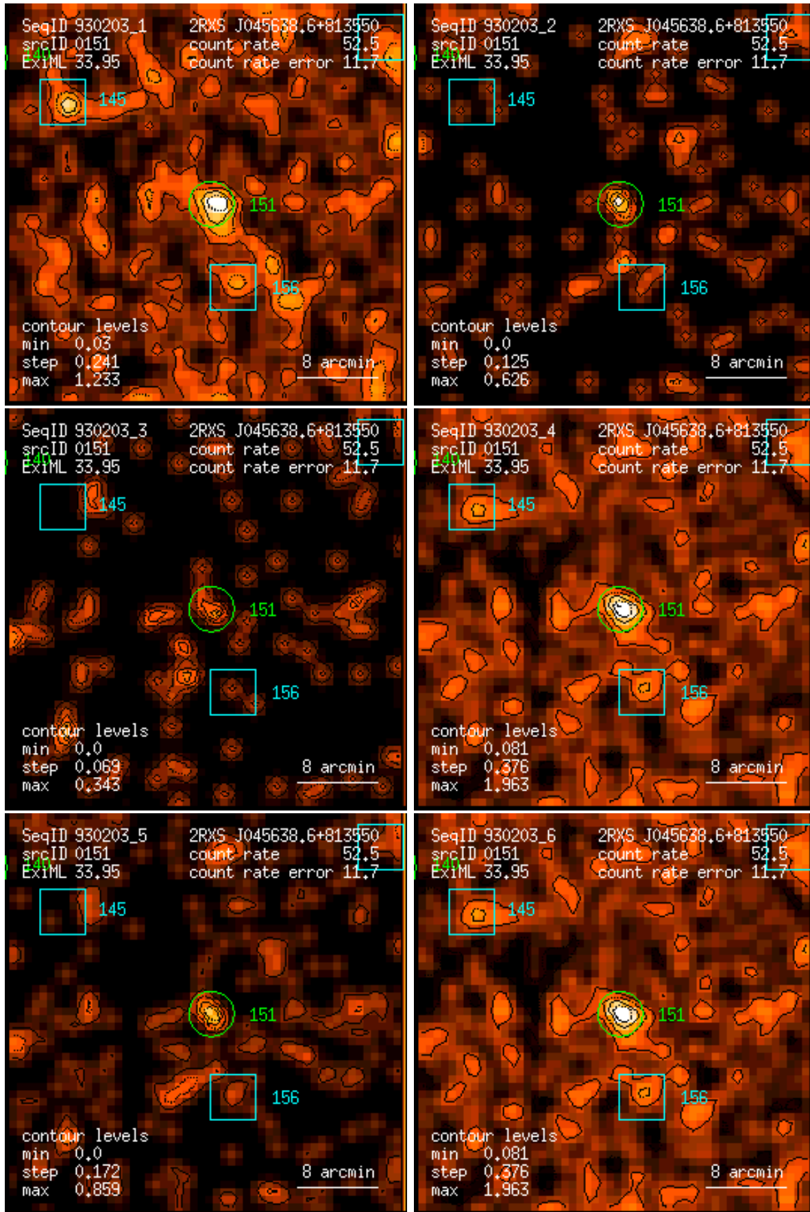
Figure 151: RASS 930203: detection 0151: band rate images, Gaussian filter: (1) PSPC channels 11 – 41, (2) 52 – 90, (3) 91 – 201, (4) 11 – 235, (5) 52 – 201, (6) 11 – 201. Broad band rates in counts/ks. Band rate contour levels in counts/ks/arcmin 2 .
