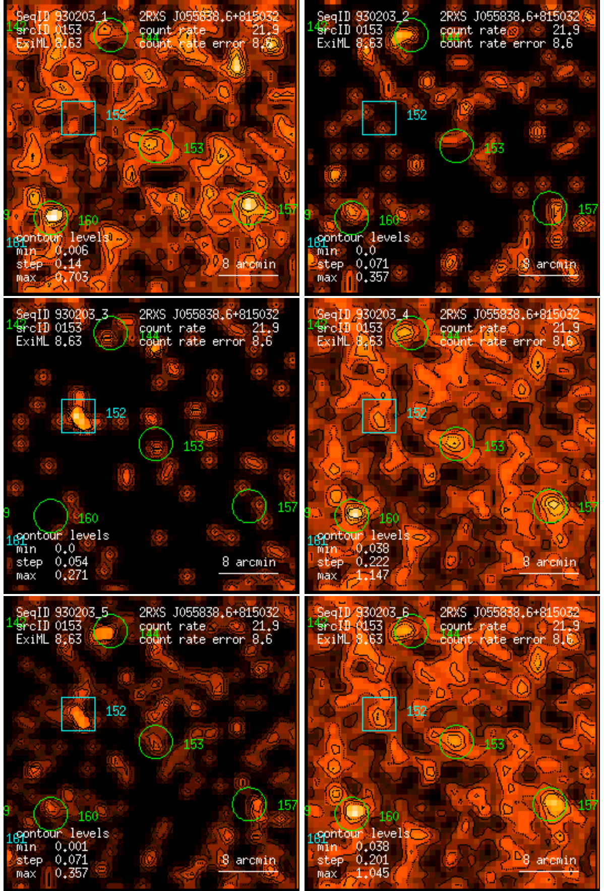
Figure 153: RASS 930203: detection 0153: band rate images, Gaussian filter: (1) PSPC channels 11 – 41, (2) 52 – 90, (3) 91 – 201, (4) 11 – 235, (5) 52 – 201, (6) 11 – 201. Broad band rates in counts/ks. Band rate contour levels in counts/ks/arcmin 2 .
